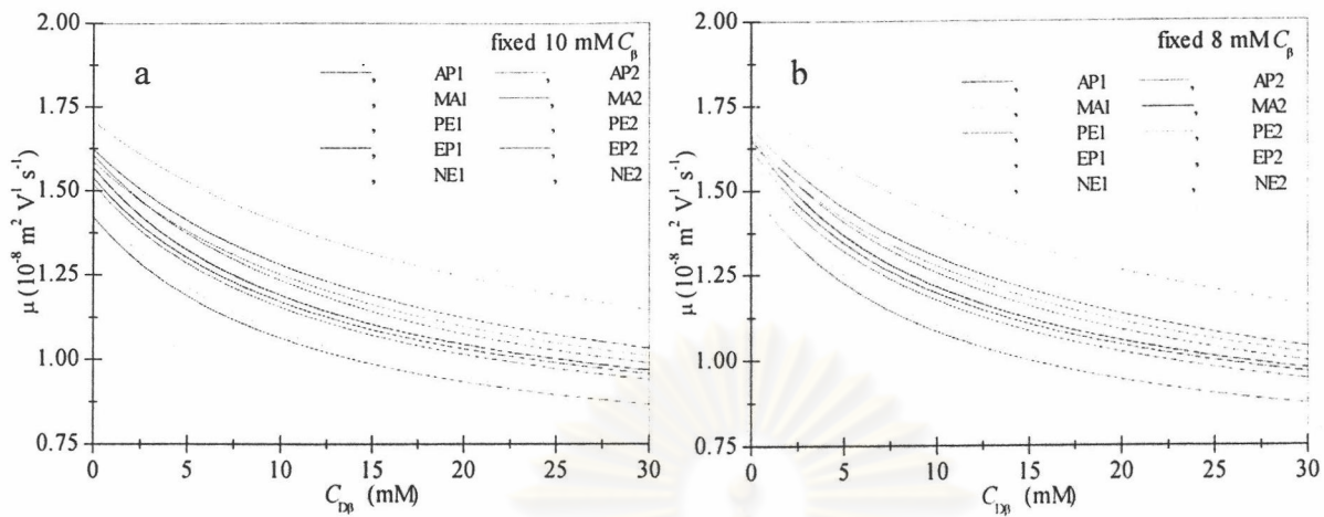
Figure 3.22 Predicted electrophoretic mobility of each enantiomer at fixed C_\beta over a wide range of C_{D\beta} . Equations from 3.16 and 3.17 and data from Table 3.1.
