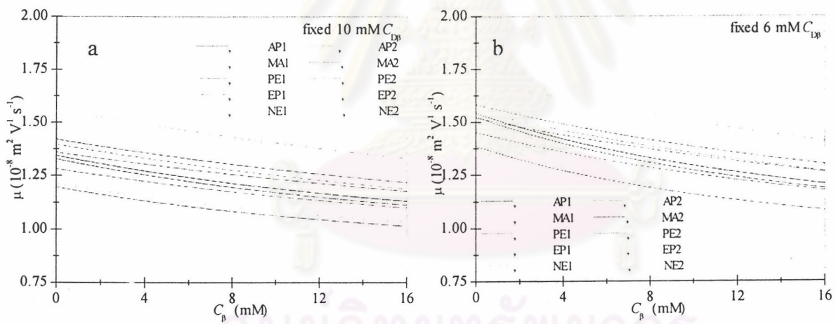
Figure 3.23 Predicted electrophoretic mobility of each enantiomer at fixed C_{D\beta} over a wide range of C_\beta . Equations from 3.16 and 3.17 and data from Table 3.1.
