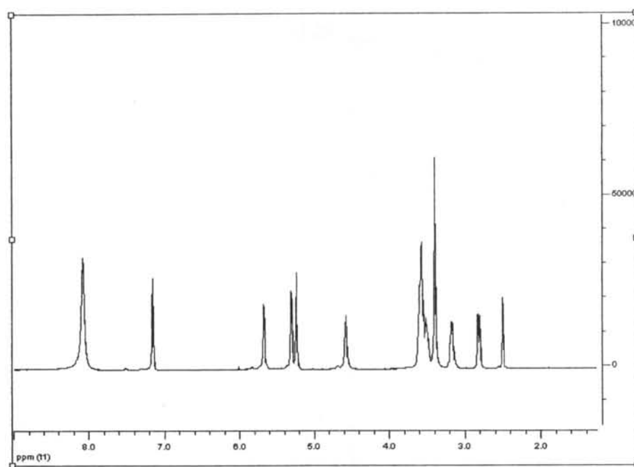
Figure 2.3 ^1\text{H} NMR of standard GlcNHCl in DMSO, \text{D}_2\text{O}
