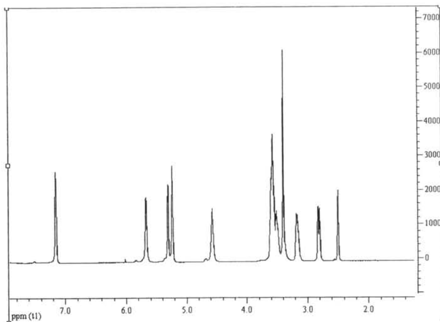
Figure 2.2 ^1\text{H} NMR of standard GlcNHCl in DMSO
