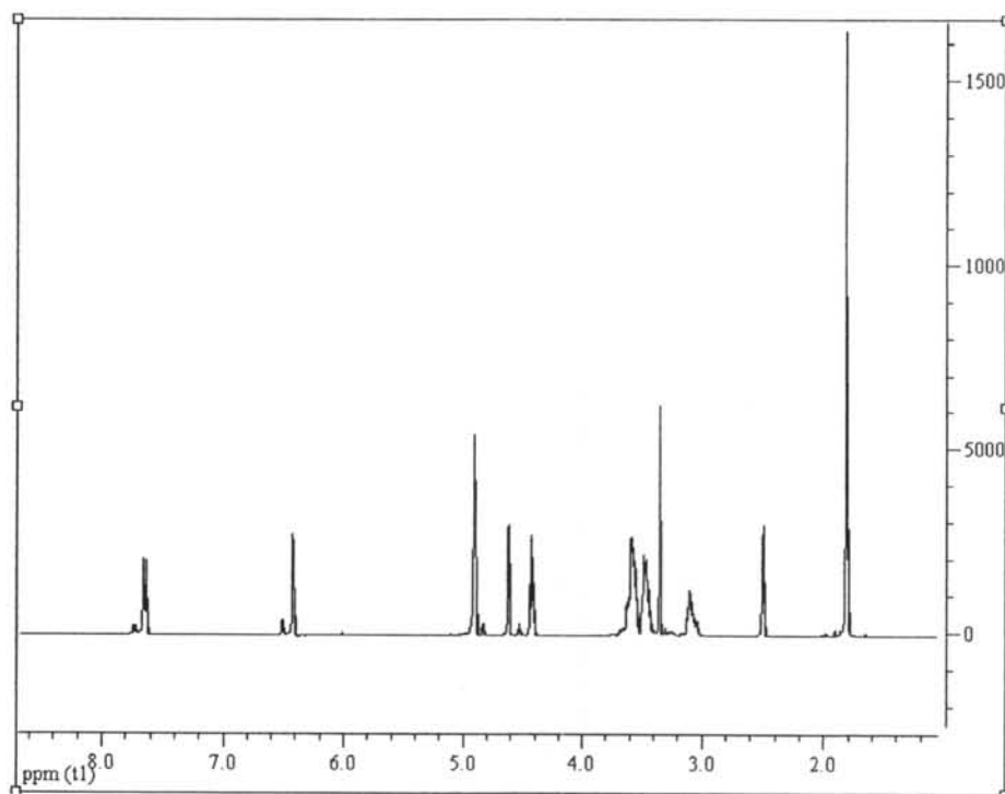
Figure 1.2 ^1\text{H} NMR of standard GlcNAc in DMSO
