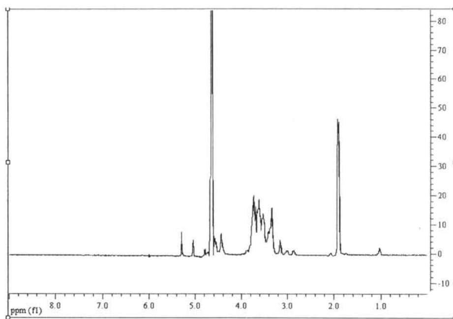
Figure 1.1 ^1\text{H} NMR of standard GlcNAc in \text{D}_2\text{O}
