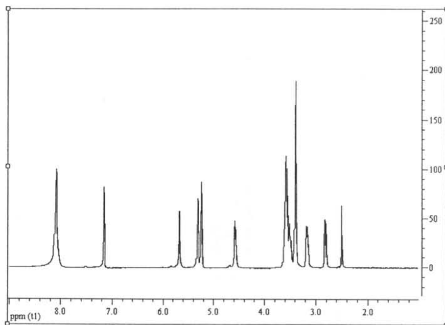
Figure 2.1 ^1\text{H} NMR of standard GlcNHCl in \text{D}_2\text{O}
