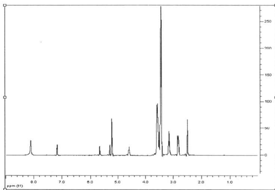
Figure 1.3 ^1\text{H} NMR of standard GlcNAc in DMSO, \text{D}_2\text{O}
