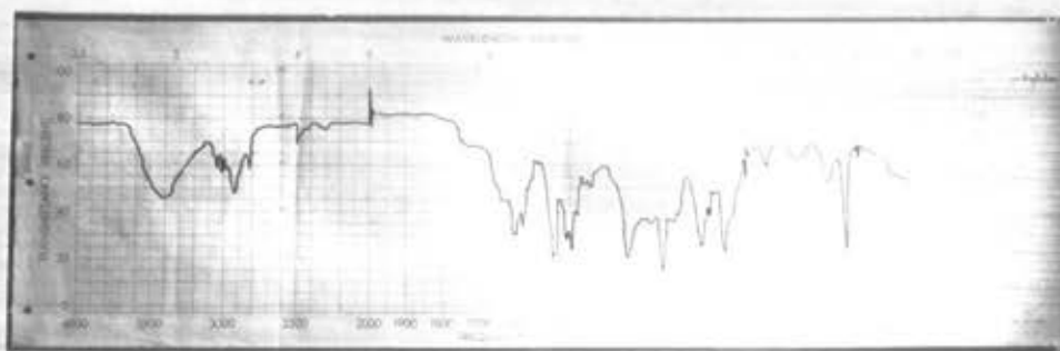
Figure 4: I.R. spectrum of the methyl derivative
