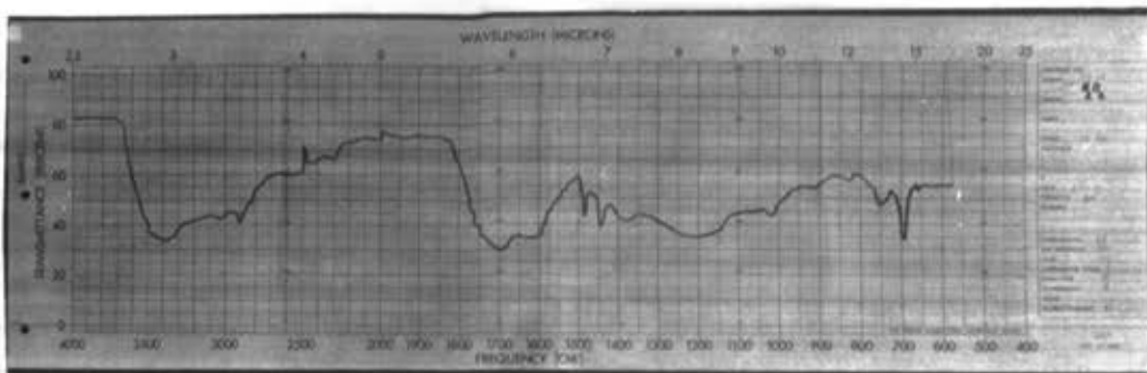
Figure 5: I.R. spectrum of the oxidation product with H_2O_2
