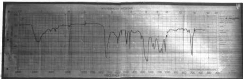
Figure 7: I.R. spectrum of the benzoyl derivative
