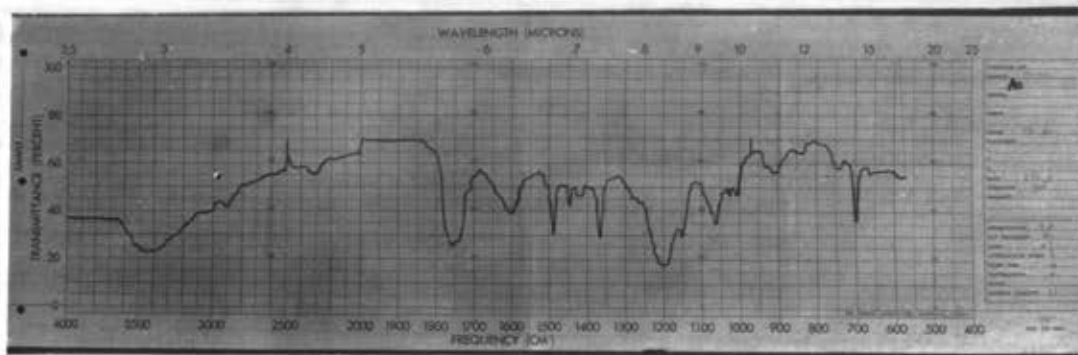
Figure 6: I.R. spectrum of the acetyl derivative
