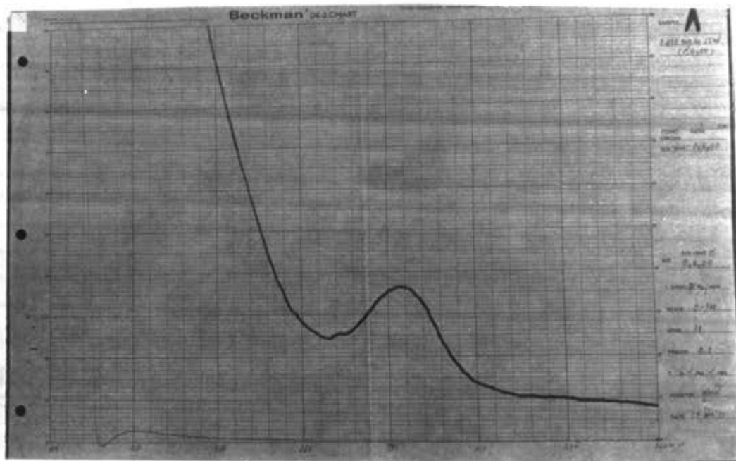
Figure 3: U.V. spectrum of thailandine
