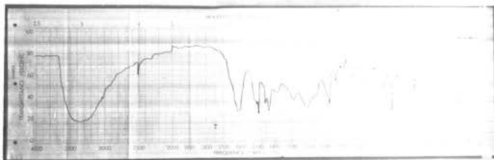
Figure 1: I.R. spectrum of thailandine
