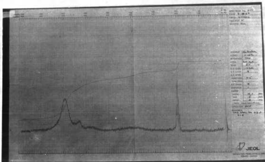
Figure 2: n.m.r. spectrum of thailandine
