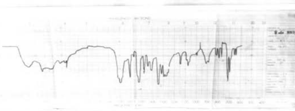
Figure 8: I.R. spectrum of the oxidation product with conc. \text{HNO}_3
