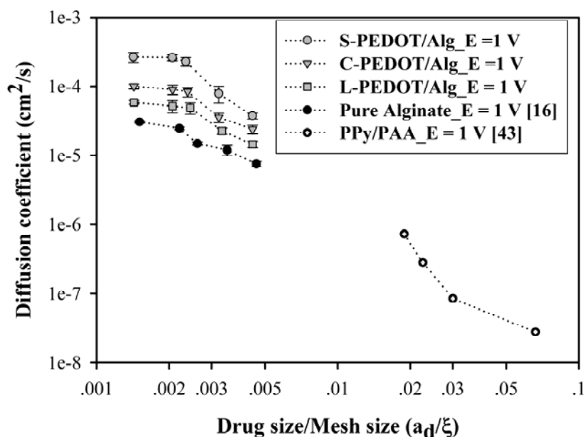
Figure 12 Diffusion coefficient of drug from alginate, PEDOT/Alg, and PPy/PAA hydrogel at electrical potential of 1 V.
