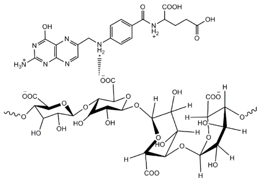
Figure 14 The interaction between folic acid and alginate.
