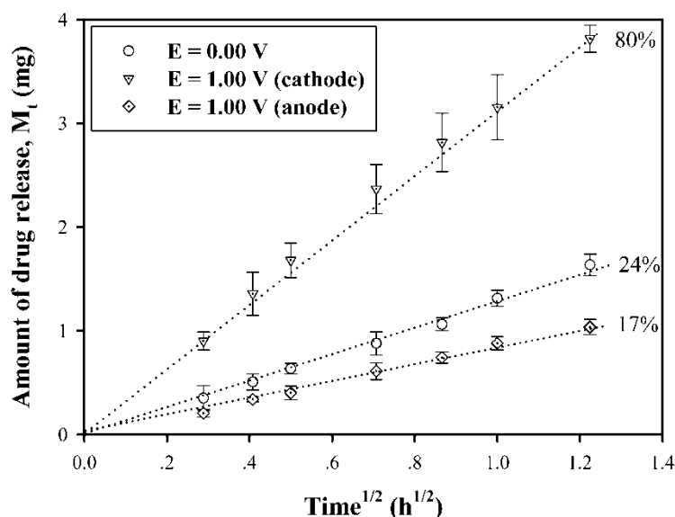
Figure 10 Amounts of benzoic acid released from S-PEDOT/Alg 0.7 hydrogels at electrical potentials of 0 V and 1 V with hydrogel samples attached to anode or cathode.
