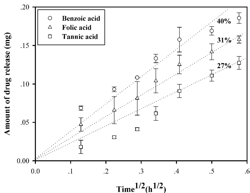
Figure 13 Amounts of drug released from Alg_0.7 hydrogels of various drug sizes versus time 1/2 .
