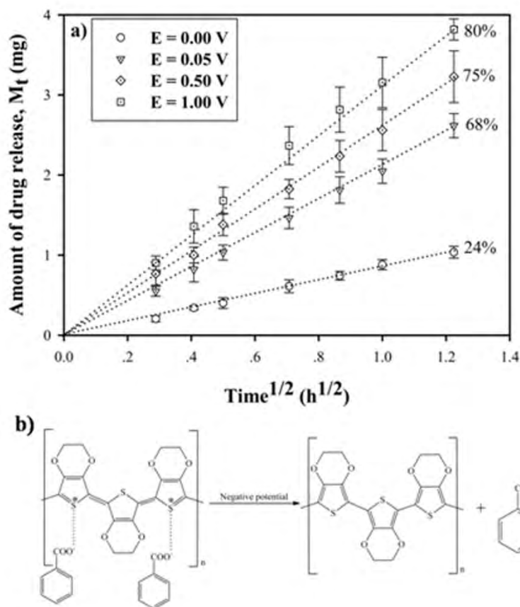
Figure 7 a) Amount of benzoic acid released from S-PEDOT/Alg 0.7 hydrogels at various electrical potentials b) Release reaction of benzoic acid from BA-loaded PEDOT/Alg hydrogel under applied electric field.
