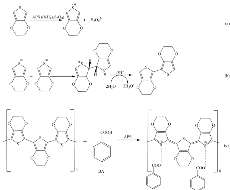
Figure 4 Proposed polymerization mechanism of BA-loaded PEDOT: (a) EDOT as a monomer is oxidized by APS to a cation radical; (b) EDOT cation radicals form dimers that subsequently are deprotonated; and (c) PEDOT polymer is doped by benzoate ion.
