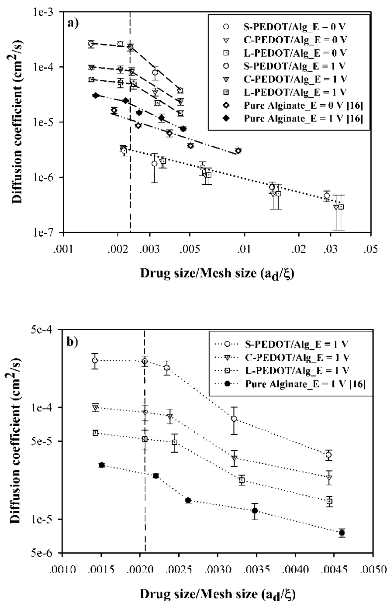
Figure 11 Diffusion coefficient of: a) benzoic acid from alginate and PEDOT/Alg hydrogel at electrical potentials of 0 and 1 V; and b) benzoic acid from PEDOT/Alg hydrogel at electrical potential of 1 V.
