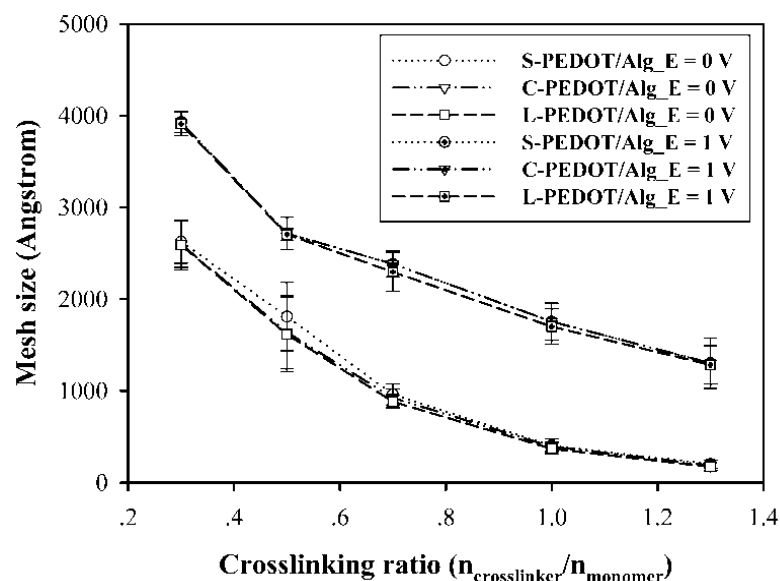
Figure 5 Mesh size of PEDOT/Alg hydrogel at various crosslinking ratios under electrical potential of 0 and 1 V.
