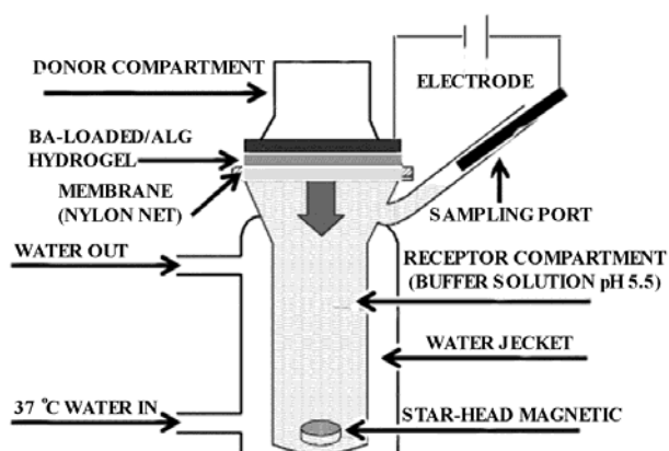
Figure 1 The modified Franz-Diffusion cell experiment set up.
