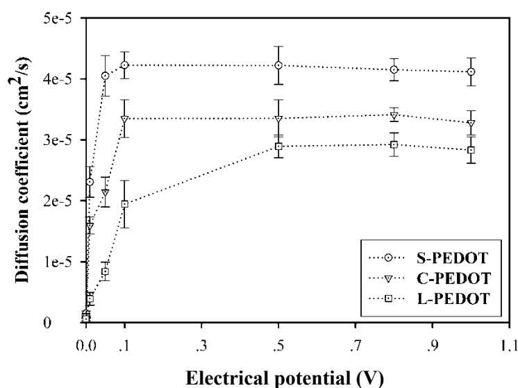
Figure 8 Diffusion coefficient of benzoic acid from PEDOT/Alg 0.7 of various PEDOT particle sizes vs. electrical potential.
