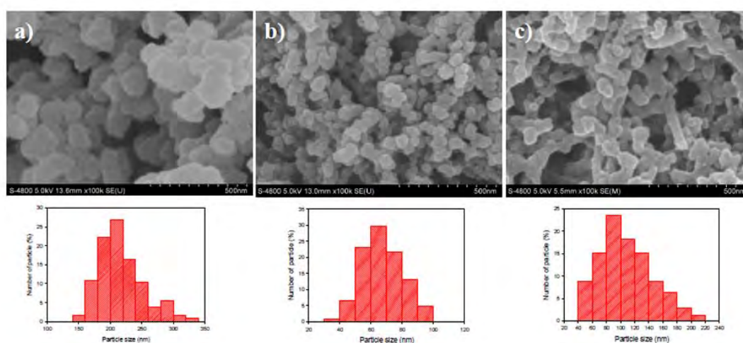
Figure 3 Morphologies and size distributions of BA-loaded PEDOT at various APS concentrations: a) 0.15 M; b) 0.30 M; and c) 0.45 M.
