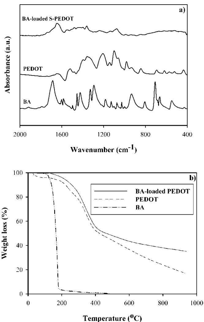
Figure 2 a) Absorption infrared spectra and b) thermogravimetric thermograms of BA, PEDOT, and BA-loaded PEDOT.
