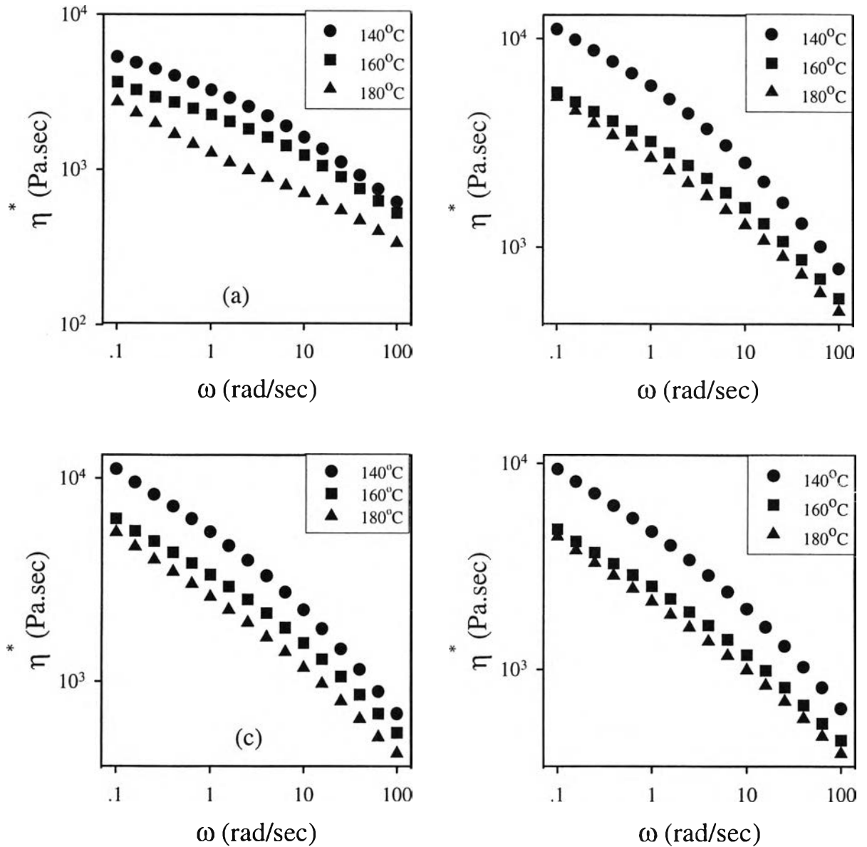
Figure A The complex viscosity as a function of frequency at different temperature for 70/30 LLDPE/NR blends at various %MA: (a) 1%MA, (b) 3%MA(c) 5%MA and (d) 7%MA
