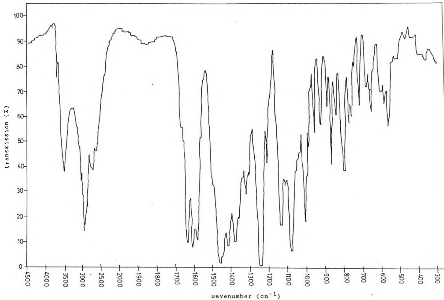
Figure 17 : Infrared absorption spectrum of A-1 in KBr disc
