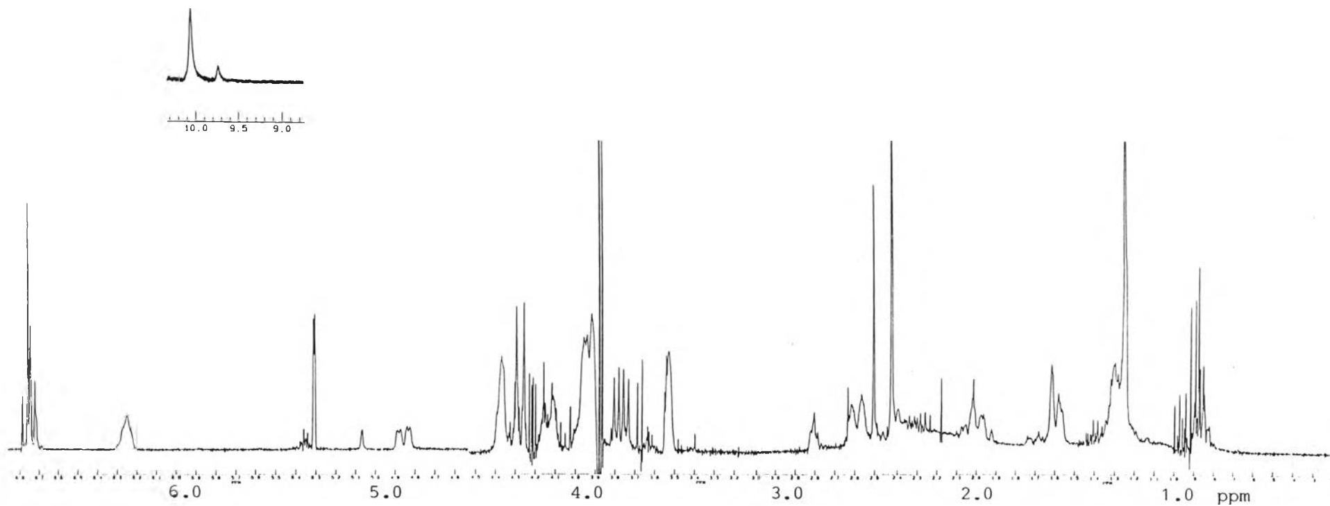
Figure 25 : ^1\text{H} Nuclear Magnetic Resonance spectrum. (300 MHz) of AA-1 in \text{CDCl}_3
