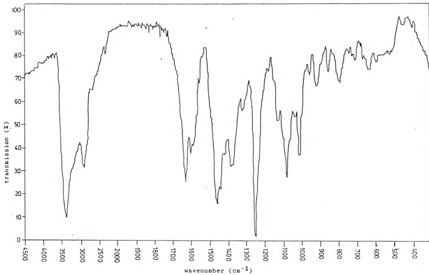
Figure 22 : Infrared absorption spectrum of AA-1 in KBr disc
