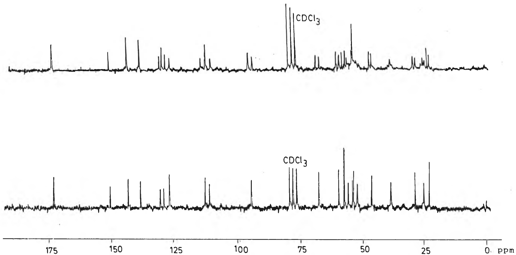
Figure 20 : ^{13}\text{C} Nuclear Magnetic Resonance spectrum (22.5 MHz) of A-1 in \text{CDCl}_3
