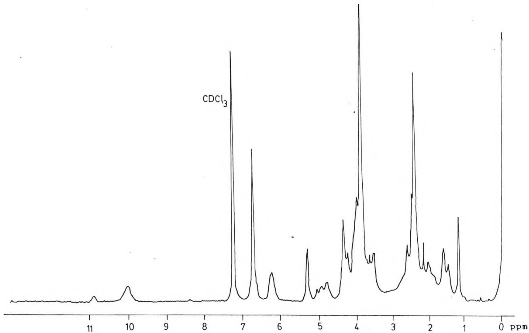
Figure 24 : ^1\text{H} Nuclear Magnetic Resonance spectrum (90 MHz) of AA-1 in \text{CDCl}_3
