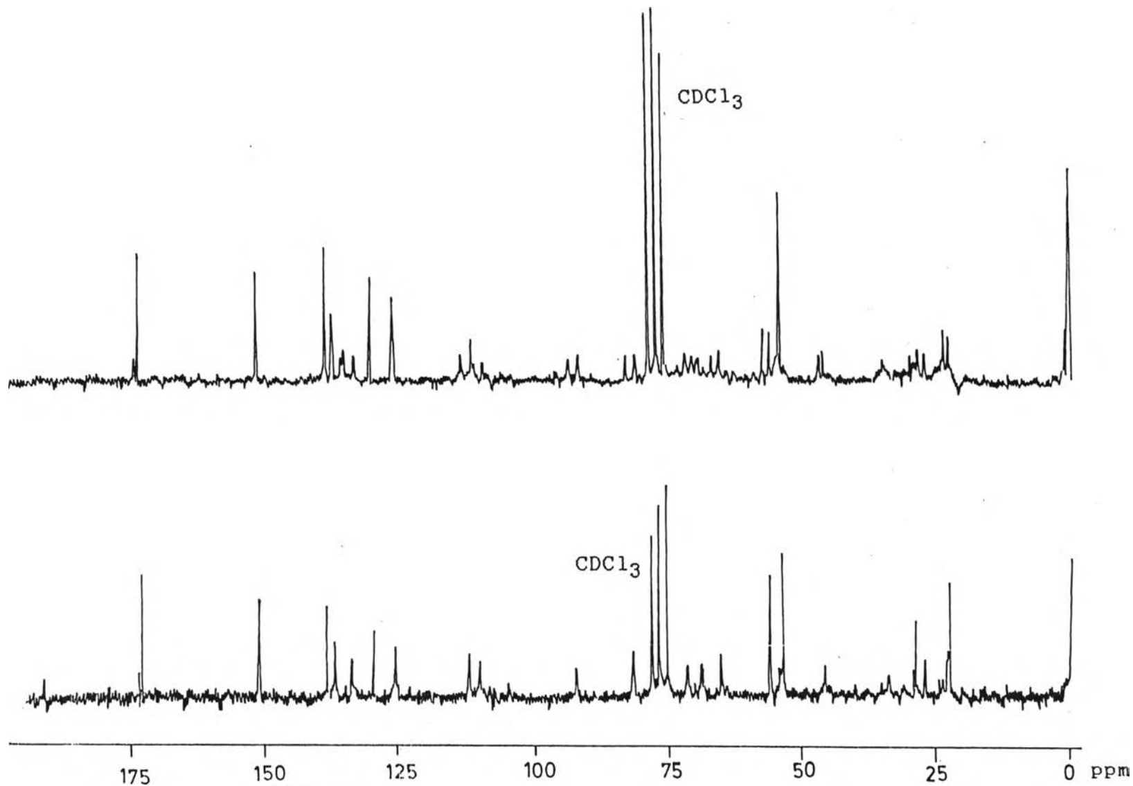
Figure 26 : ^{13}\text{C} Nuclear Magnetic Resonance spectrum (22.5 MHz) of AA-1 in \text{CDCl}_3
