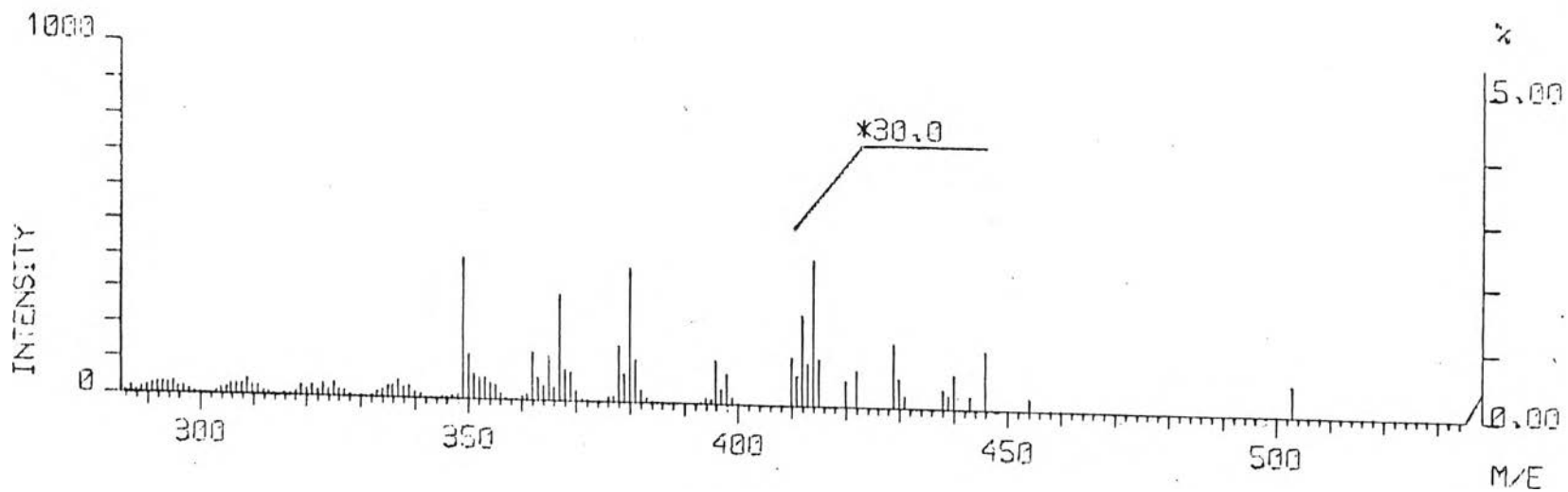
Figure 23 : Mass spectrum of AA-1
