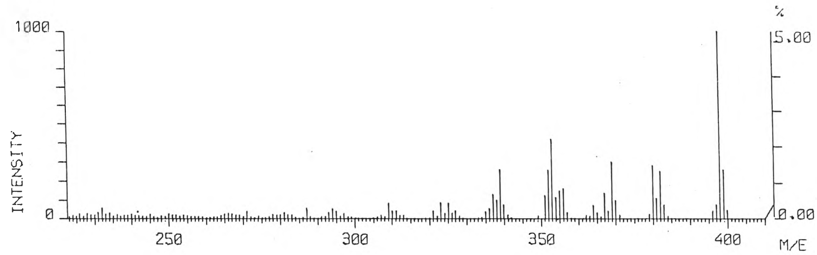
Figure 18 : Mass spectrum of A-1
