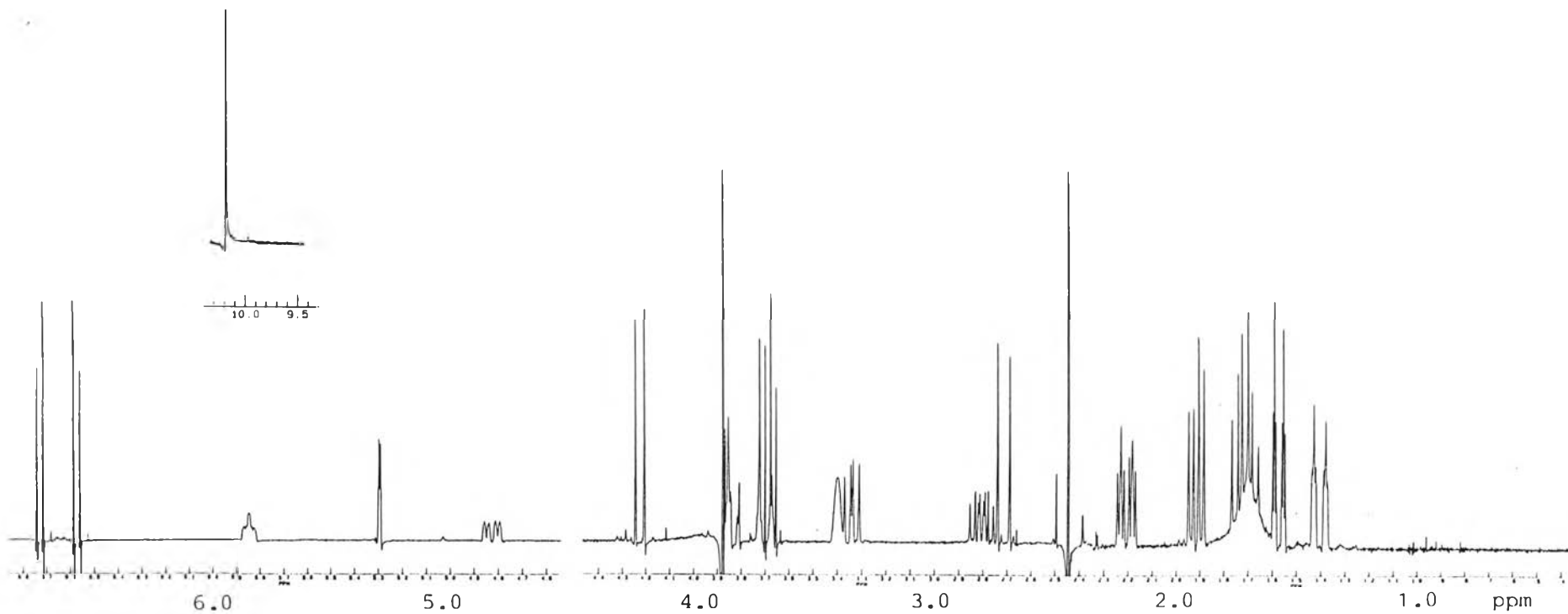
Figure 19 : ^1\text{H} Nuclear Magnetic Resonance spectrum (300 MHz) of A-1 in \text{CDCl}_3
