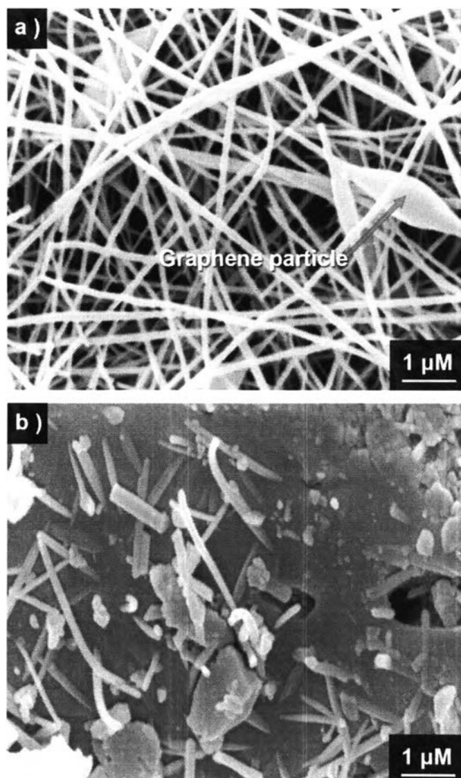
Figure 4.2 (a) SEM image of PAN5G before carbonization and (b) SEM image of CPAN5G after carbonization
