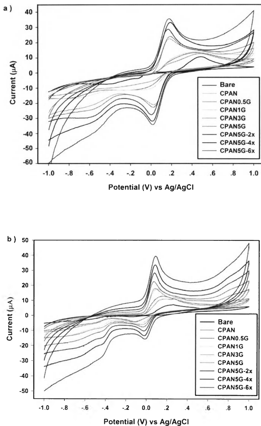
Figure 4.4; CV of 0.1 M PBS at a pH of 7.4 at unmodified/modified electrodes with a scan rate of 50 \text{mV s}^{-1} in, (a) in 1 mM [\text{Fe}(\text{CN})_6]^{3-/4-} and (b) in 40 \mu\text{M} DA.
