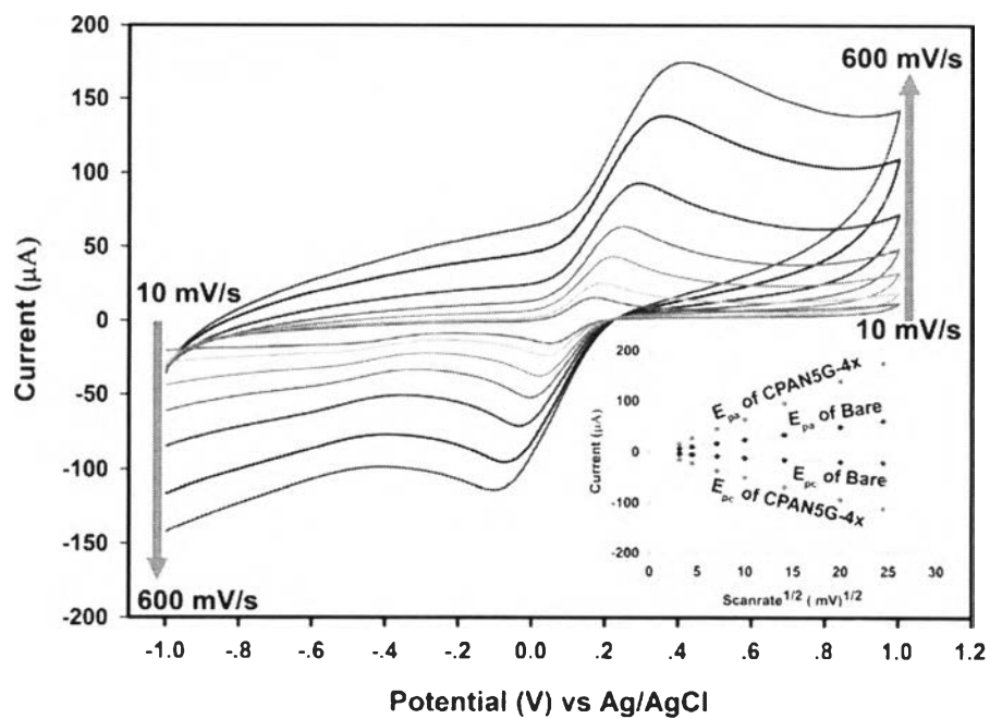
Figure 4.5 CV of 1 mM [\text{Fe}(\text{CN})_6]^{3-/4-} in 0.1 M PBS at a pH of 7.4 at different scan rates at of the CPAN5G-4x electrode measured using. Inset is the plot of the linear relationship between the current and scan rate 1/2 for the bare and CPAN5G-4x electrodes.
