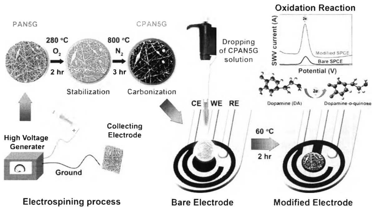
Figure 4.1 Schematic of SPCE surface modifications
