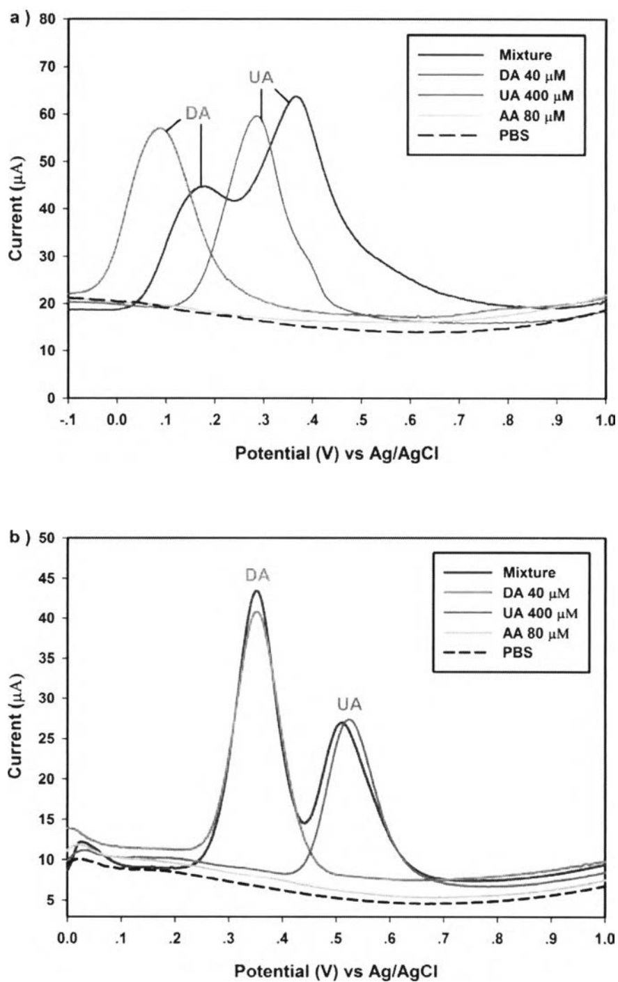
Figure 4.8 SWV of 0.1 M PBS/5 mM SDS at a pH of 2. SWV detection conditions: pulse amplitude=0.06 V, square wave frequency=18 Hz, and step height=0.005 V
