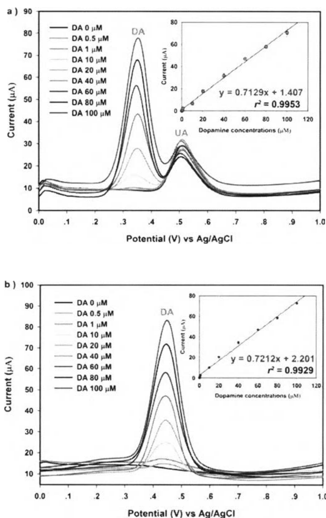
Figure 4.9 (a) Representative SWV of 0.1 M PBS/5 mM SDS at a pH of 2 at the CPAN5G-4x electrode; The inset of (a) is the calibration curve for DA detection over a concentration range of 0.5-100 \mu\text{M} in the presence of AA and UA at 80 and 400 \mu\text{M} , respectively; (b) Representative SWV profiles of the CPAN5G-4x electrode in human serum after TCA protein precipitation; The inset of (b) is the calibration for different spiked DA concentrations over the range of 0.5-100 \mu\text{M} .
