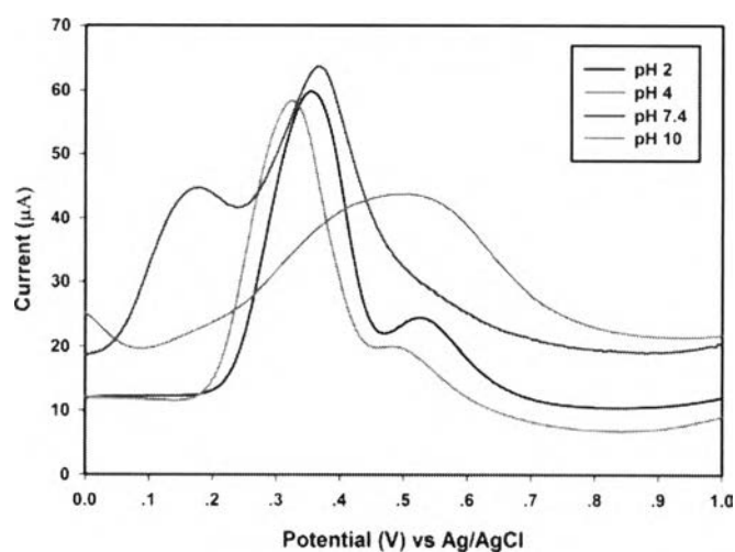
Figure 4.11 SWV of 40 \text{ } \mu\text{M} DA, 80 \text{ } \mu\text{M} AA, and 400 \text{ } \mu\text{M} in 0.1 M PBS/5 mM SDS at various pH conditions. SWV detection conditions: pulse amplitude= 0.06 \text{ V} , square wave frequency= 18 \text{ Hz} , and step height= 0.005 \text{ V} .
