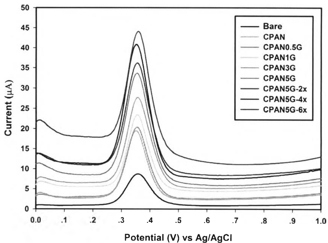
Figure 4.7 SWV of 40 \mu\text{M} of DA in 0.1 M PBS/5 mM SDS at a pH of 2 at unmodified and modified. SWV detection conditions: pulse amplitude=0.06 V, square wave frequency=18 Hz, and step height=0.005 V.
