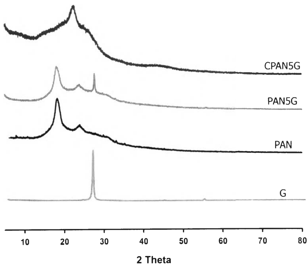
Figure 4.3 XRD patterns of G, PAN, PAN5G, and CPAN5G nanofibers
