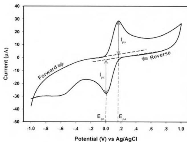
Figure 4.10 CV showing I_{pa} , I_{pc} , E_{pa} and E_{pc} using CPAN5G-4x electrodes with a scan rate of 50 \text{ mV s}^{-1} in 0.1 M PBS at a pH of 7.4 in 1 \text{ mM } [\text{Fe}(\text{CN})_6]^{3-/4-}
