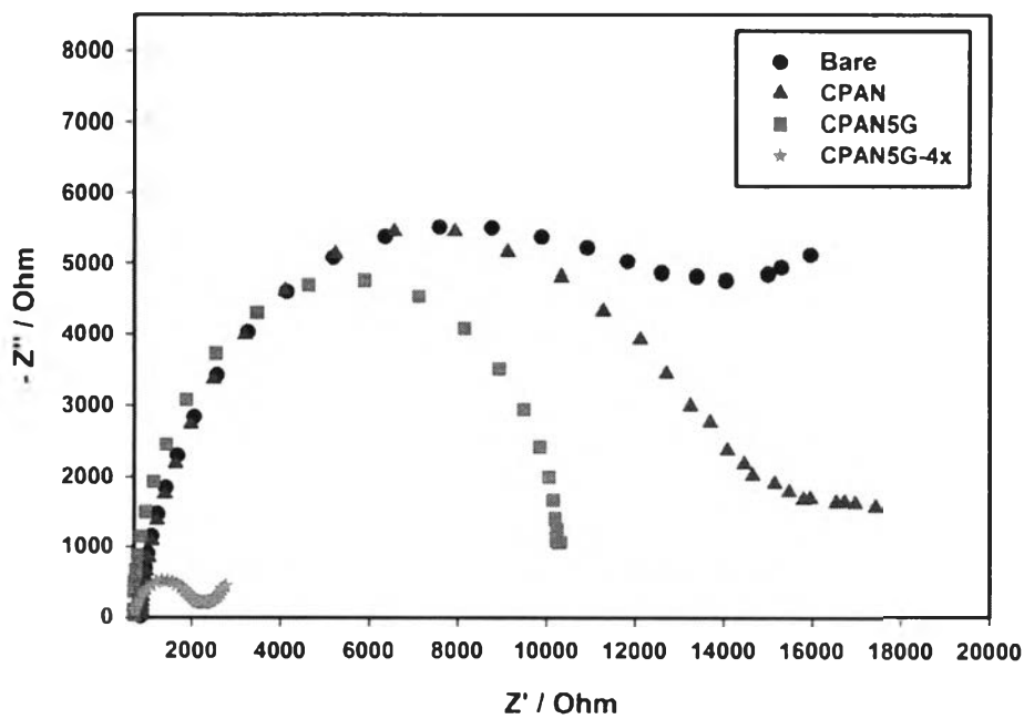
Figure 4.6 EIS using BARE, CPAN, CPAN5G, and CPAN5G-4x in 1 mM [\text{Fe}(\text{CN})_6]^{3-/4-} in the presence of 0.1 M PBS at a pH of 7.4
