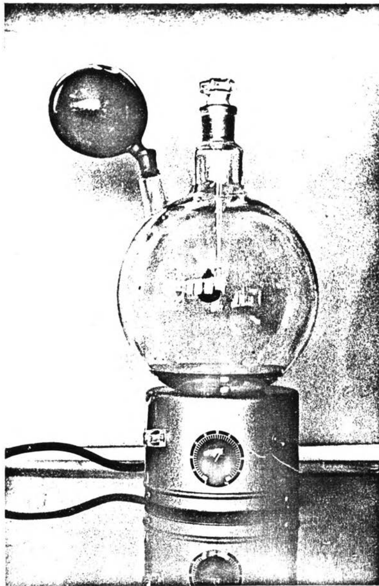
Figure 3-3 COMBUSTION FLASK WITH PLATINUM HOLDER.
