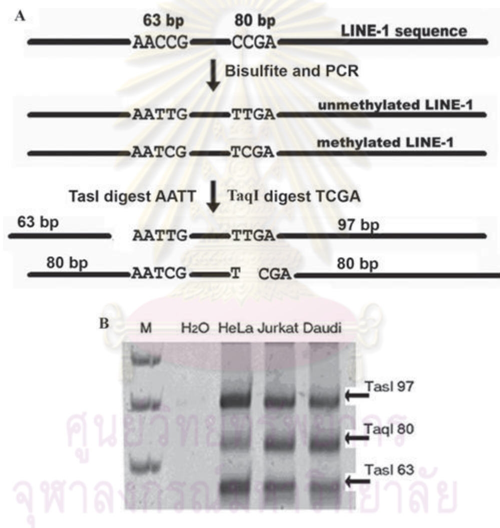
Fig. 2 Combined bisulfite restriction analysis of LINE-1 (COBRA LINE-1) [3]. LINE-1 methylation level was calculated as a percentage of intensity of TaqI divided by the sum of TaqI - and TasI -positive amplicons. (A) Schematic illustration of COBRA LINE-1. The LINE-1 amplicon size is 160 bp. Methylated amplicons, TaqI positive, yielded two 80 bp DNA fragments, whereas unmethylated amplicons, TasI positive, yielded 63 and 97 bp fragments. (B) An example of COBRA LINE-1. M, 10-bp DNA size marker; numbers under each sample, methylation levels; TasI 63 and 97, unmethylated amplicons; TaqI 80, methylated amplicons. H 2 O is water, HeLa, Jurkat and Daudi are cell lines. HeLa LINE-1s are the most hypomethylated among the three.
