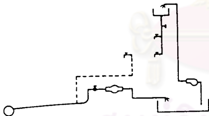
Figure I-13: Bypass supplies all water to some outlets, with service valve open or closed. During check, when service valve and storage exit valve are both closed, water still flows from illegal outlet/s. Bypass is connected upstream of the service valve. This case is more prevalent than Figure 14.
