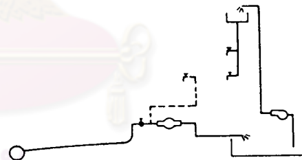
Figure I-14: Bypass supplies all water to some outlet/s when the service valve is open, no water when it is closed. During check, when service valve is closed water flow stops at illegal outlet/s only. Bypass is connected downstream of service valve.
