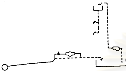
Figure I-11: Bypass supplies all water to storage when valve is closed, a portion when valve is open. During check, when valve is closed water still flows to ground storage to replenish drawdown. Bypass is connected upstream of the valve. This case is more prevalent than that in Figure 12.
