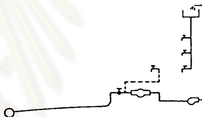
Figure I-18: Same case as Figure 14, except no sump. Check same as Figure 14.
