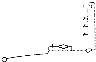
Figure I-15: Same case as Figure 11, except there is no ground storage tank (sump). Check is same as for Figure 11, except check for flow into elevated tank. This case is more prevalent than Figure 16.
