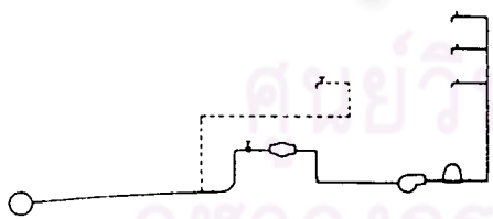
Figure I-19: Bypass supplies all water to some outlets when service valve is open or closed. During check, when pump is switched off and pressure tank is emptied only illegal outlet/s continue to flow.
