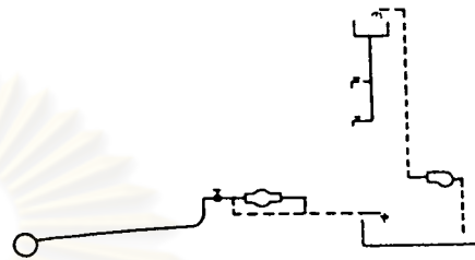
Figure I-12: Bypass supplies a portion of the water to storage when the valve is open, supplies no water when the valve is closed. The bypass can not be checked for by closing the valve; the meter must be removed and the service pipe flanged or plugged. When this is done water continues to flow to ground storage to replenish drawdown. An alternate check would be compare water volume drawn into the sump with meter registration
