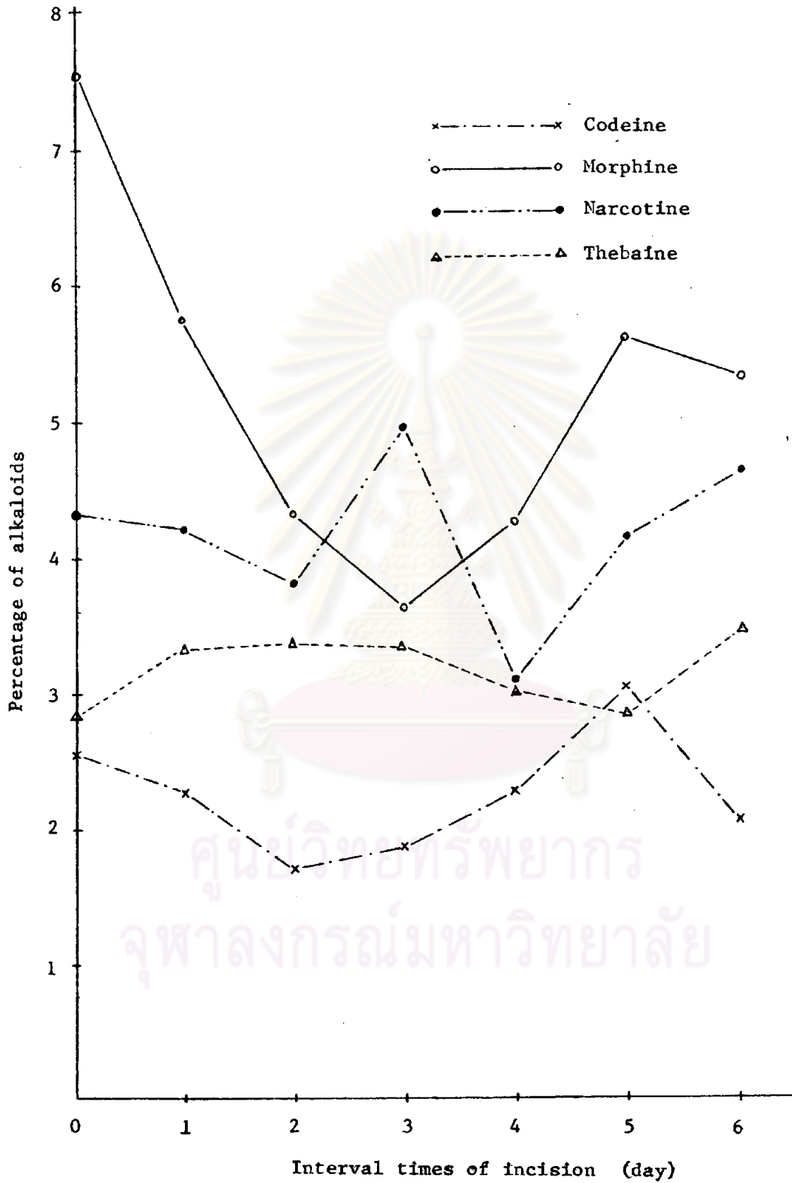
Figure 4. Alkaloidal pattern in the latex of P & TP/R
