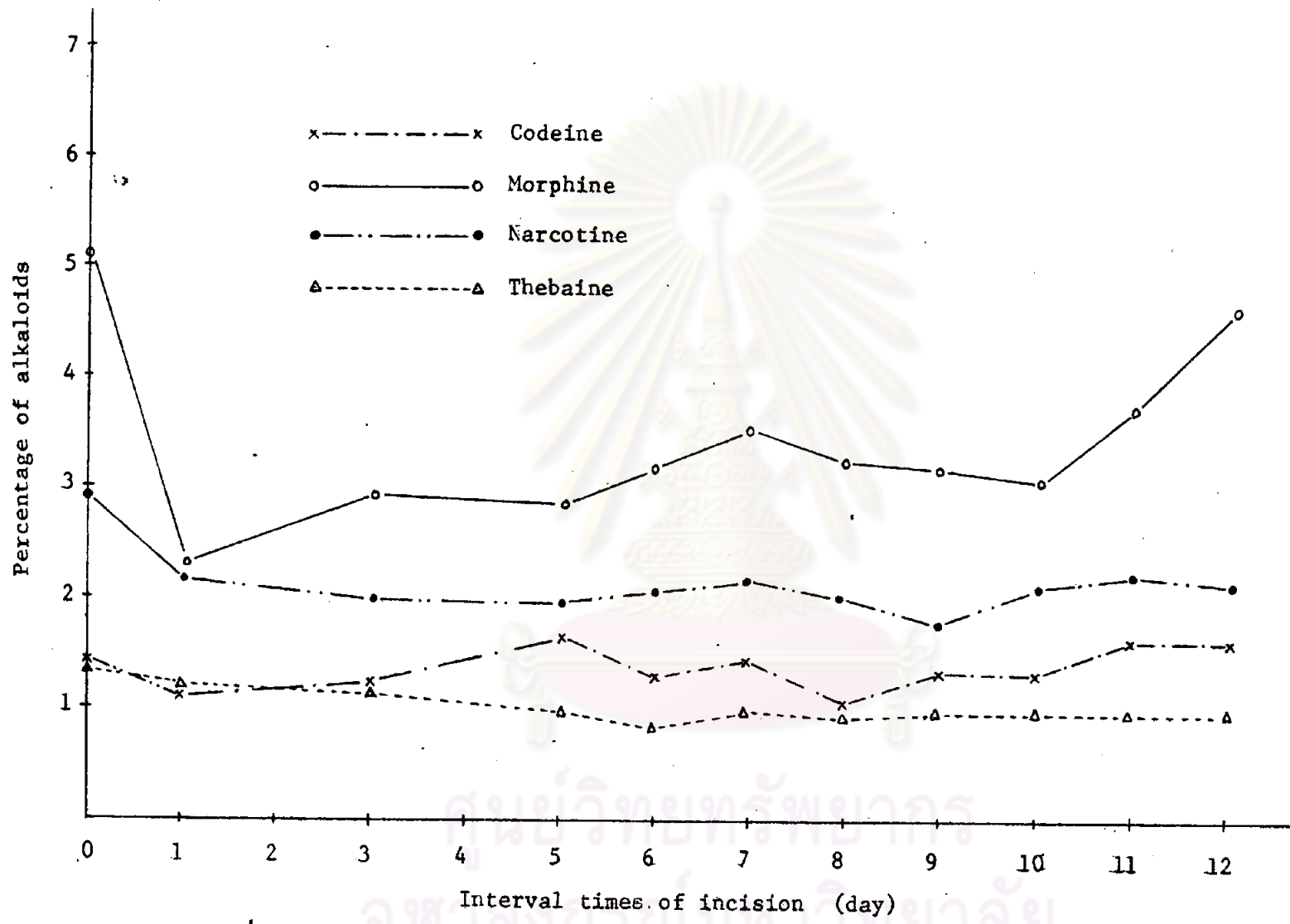
Figure 6. Alkaloidal pattern in the latex of BP & HS/R
