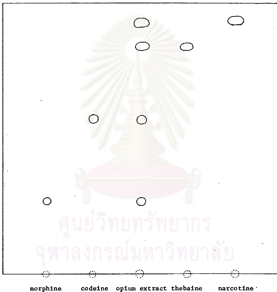
Figure 2. Thin layer chromatogram of main alkaloids from the latex of Papaver somniferum L.
