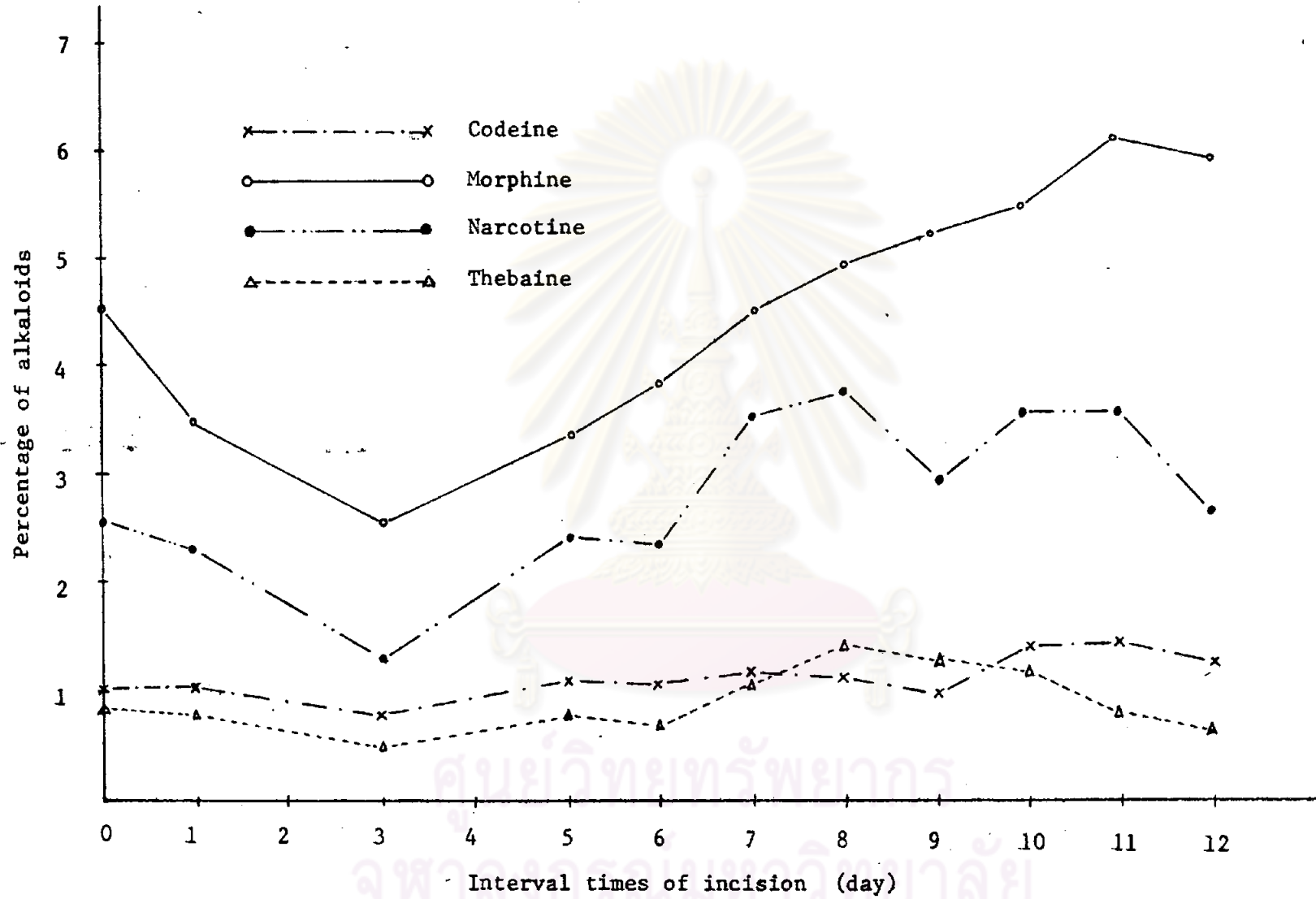
Figure 5. Alkaloidal pattern in the latex of BP & HS/W
