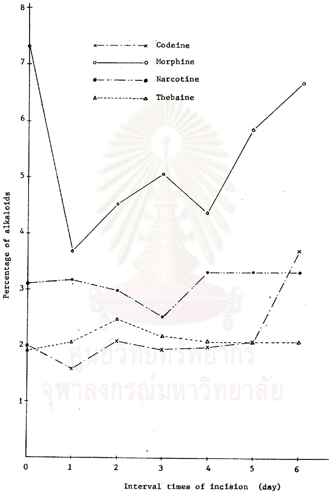
Figure 3. Alkaloidal pattern in the latex of P & TP/W
