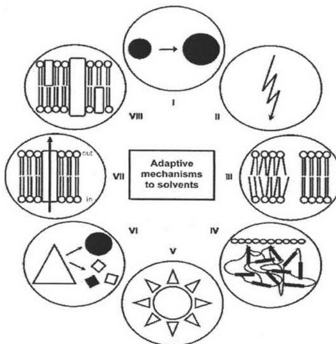
Fig.2.1 Adaptive mechanisms protecting cells against toxic effects of organic solvents.
