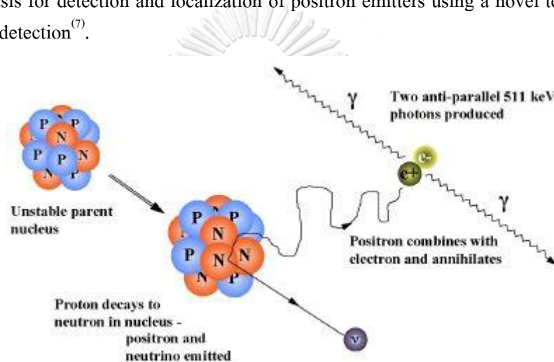
Figure 2 Positron emission and annihilation (8) .
