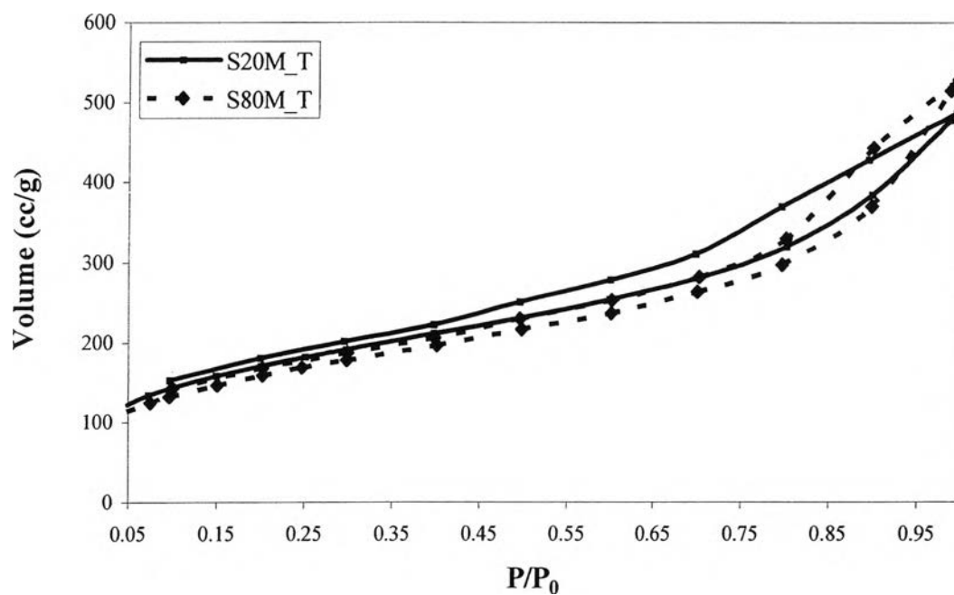
Figure 4.3 N 2 adsorption/desorption isotherm of poly(DVB)polyHIPE.
