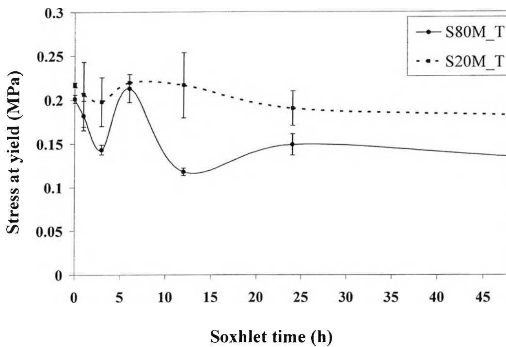
Figure 4.7 Effect of Soxhlet extraction time on compression stress of poly(DVB)polyHIPE.
