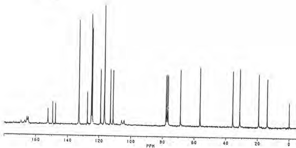
Fig 15 The ^{13}\text{C-NMR} spectrum of Compound 30
