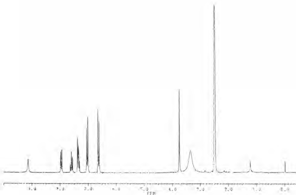
Fig 48 The 1 H-NMR spectrum of Compound R12
