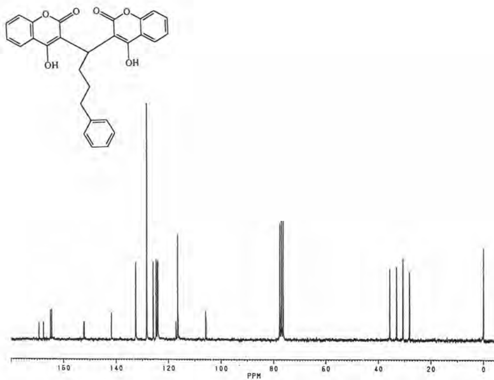
Fig 35 The ^{13}\text{C} -NMR spectrum of Compound 44
