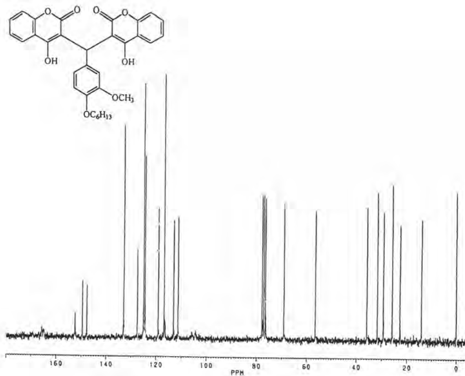
Fig 19 The ^{13}\text{C} -NMR spectrum of Compound 31
