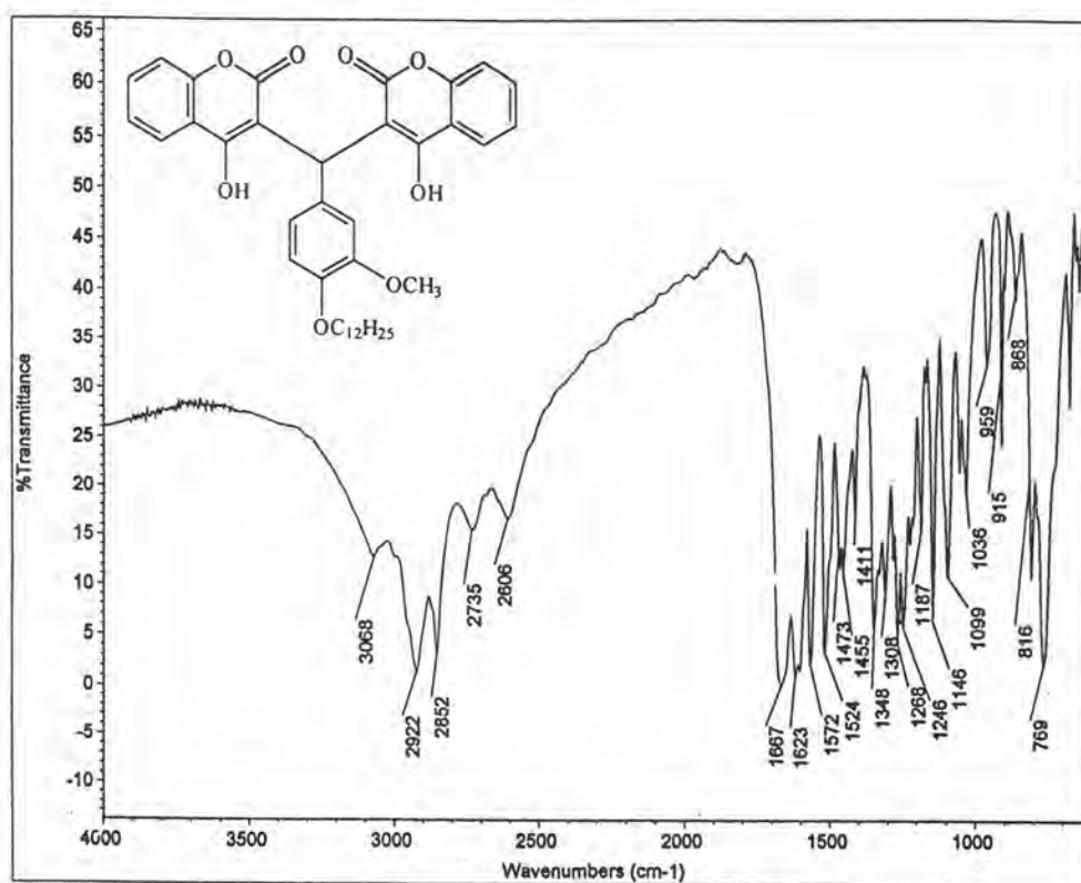
Fig 25 The FT-IR spectrum of Compound 33
