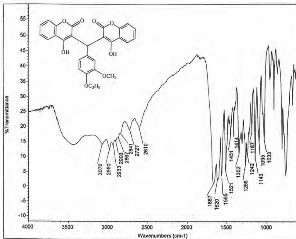
Fig 9 The FT-IR spectrum of Compound 29
