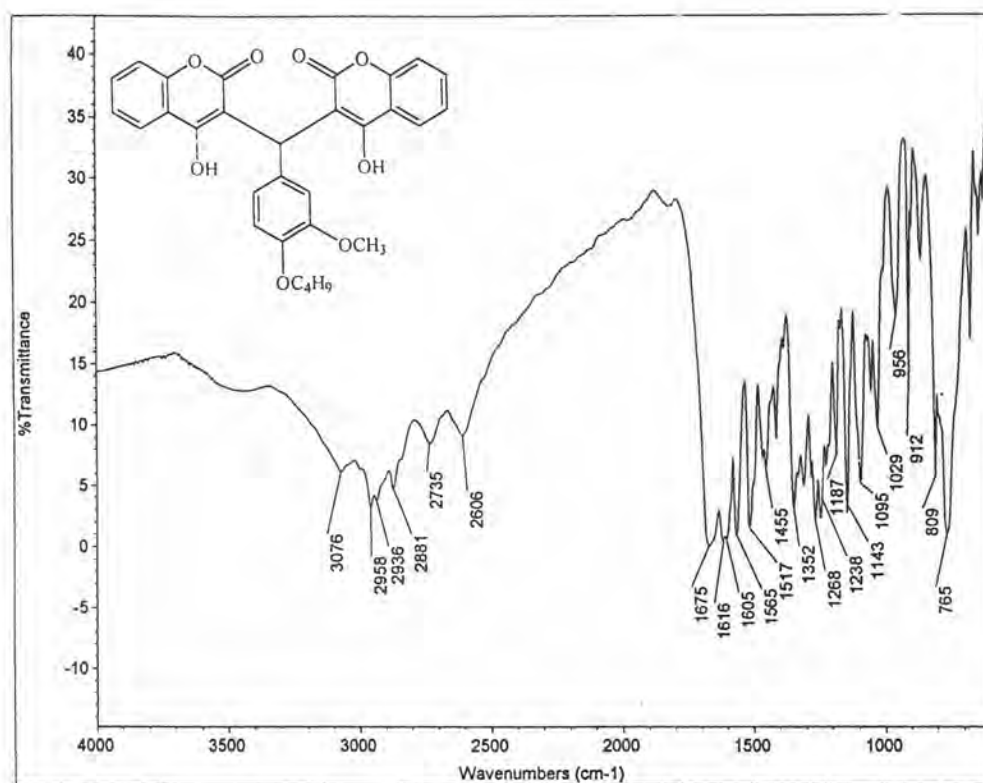
Fig 13 The FT-IR spectrum of Compound 30
