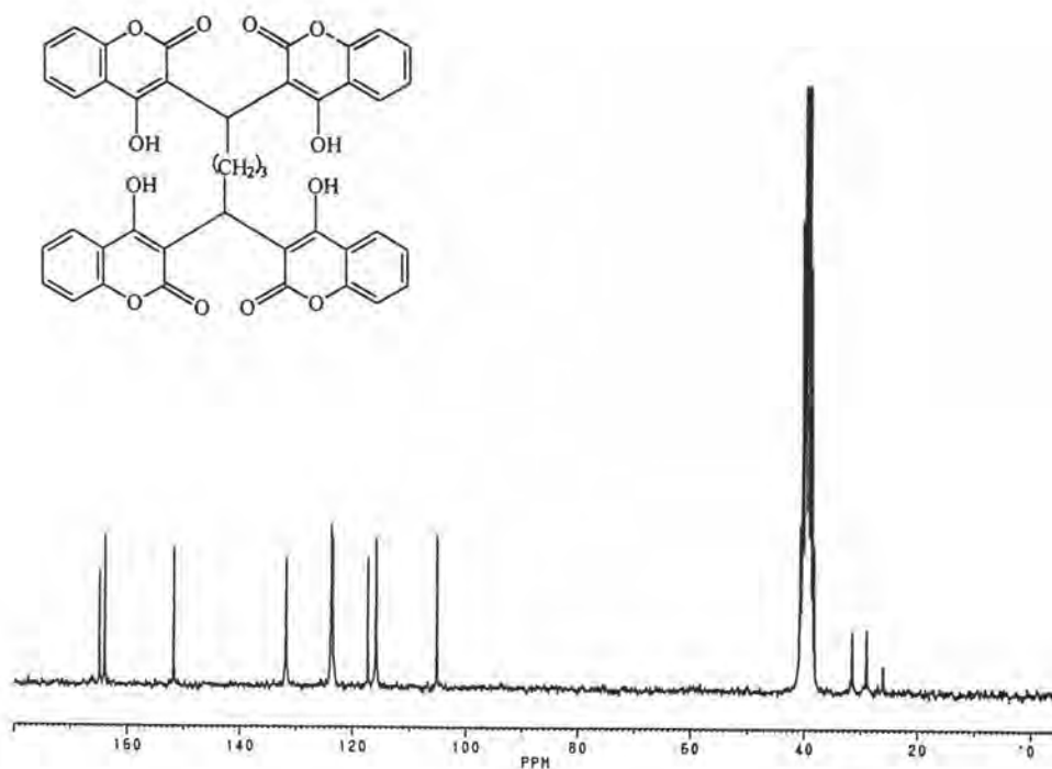
Fig 39 The ^{13}\text{C} -NMR spectrum of Compound 50
