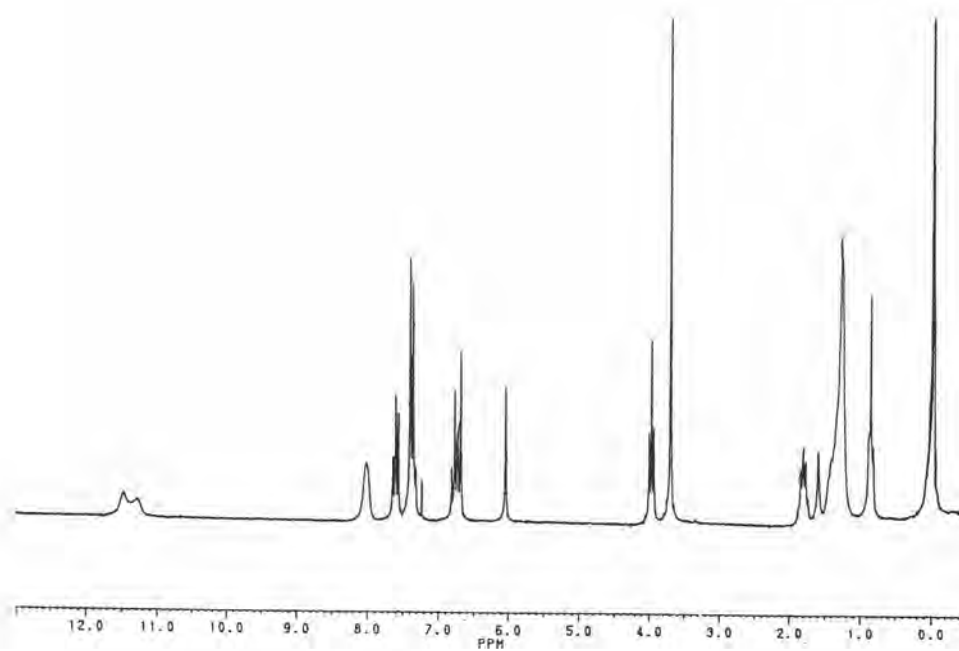
Fig 22 The 1 H-NMR spectrum of Compound 32
