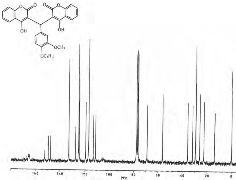
Fig 23 The ^{13}\text{C} -NMR spectrum of Compound 32
