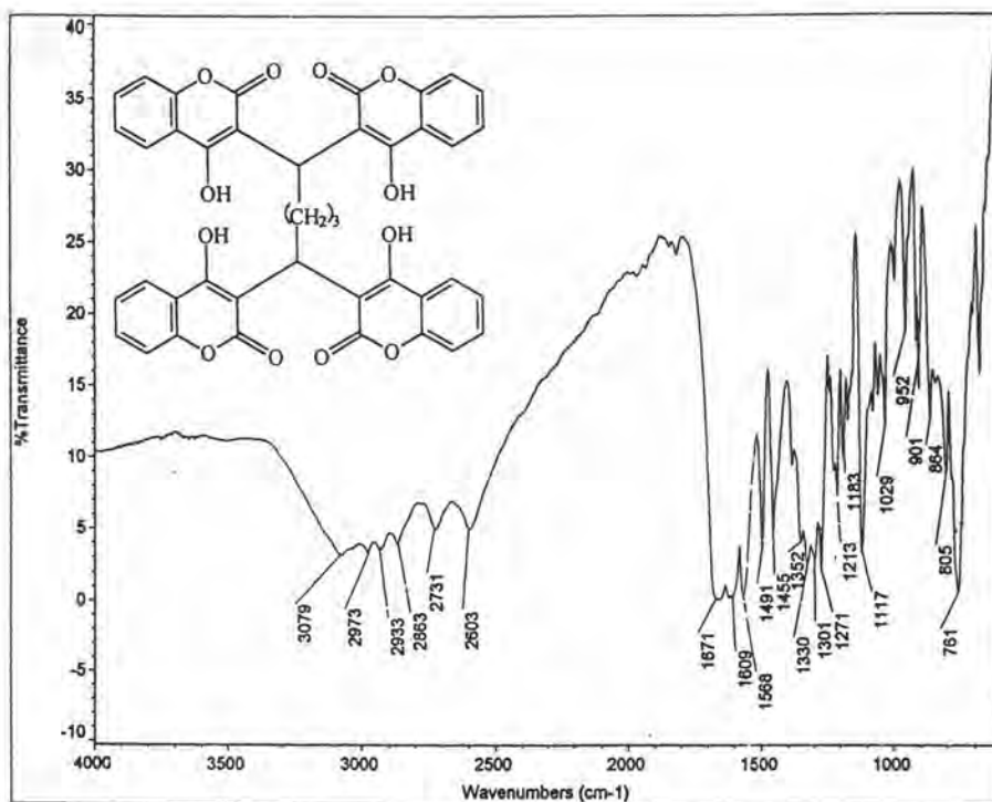
Fig 37 The FT-IR spectrum of Compound 50
