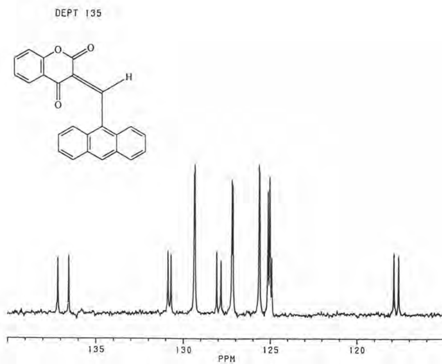
Fig 45 The DEPT 135 spectrum of Compound 54
