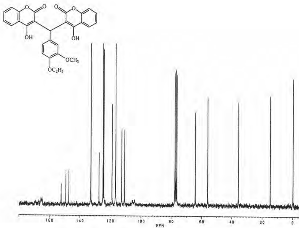
Fig 11 The ^{13}\text{C} -NMR spectrum of Compound 29
