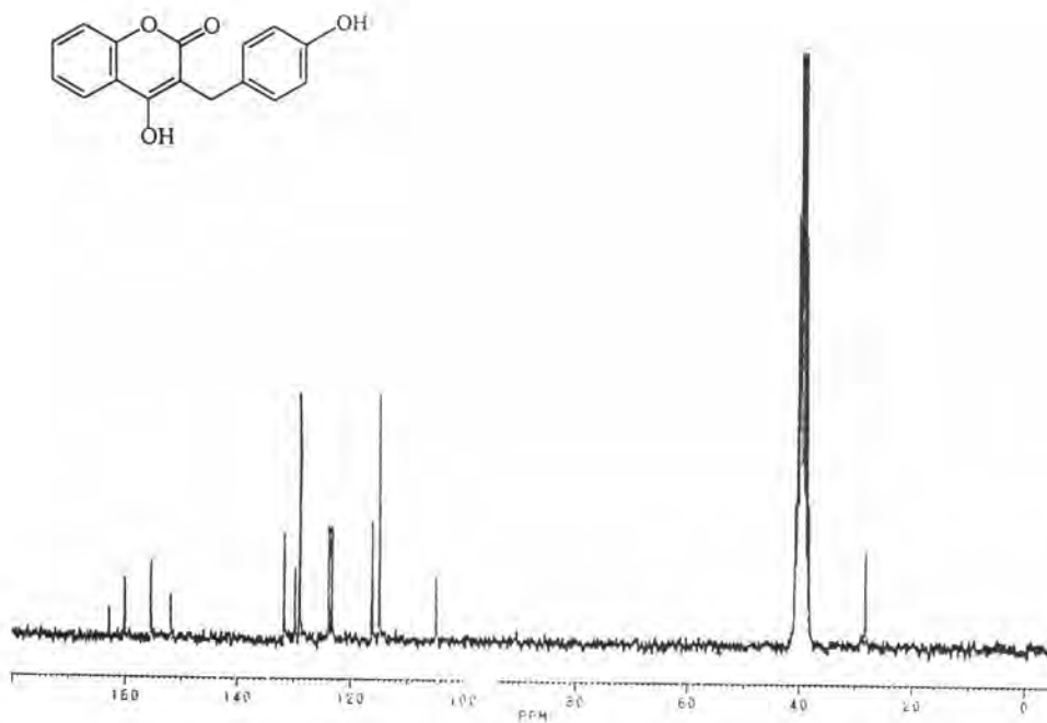
Fig 49 The ^{13}\text{C} -NMR spectrum of Compound R12
