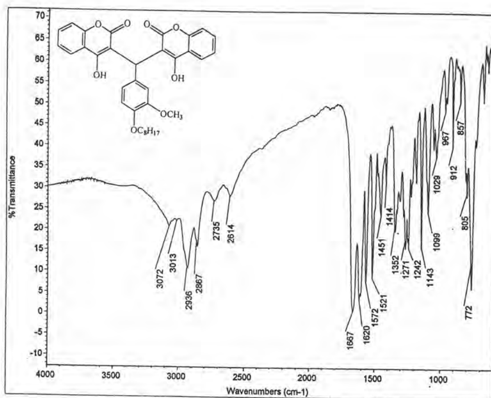
Fig 21 The FT-IR spectrum of Compound 32
