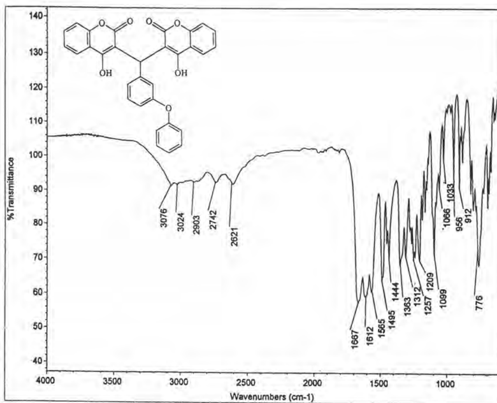
Fig 5 The FT-IR spectrum of Compound 23
