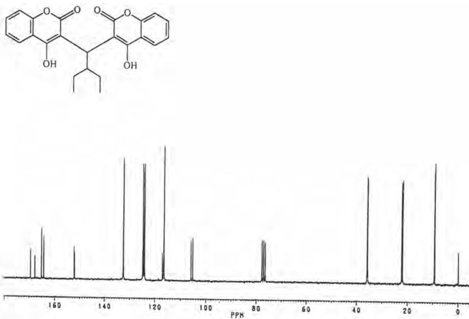
Fig 31 The ^{13}\text{C} -NMR spectrum of Compound 38
