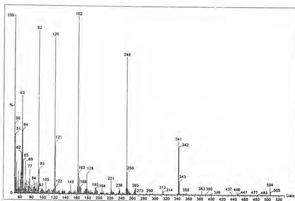
Fig 8 The mass spectrum of Compound 23
