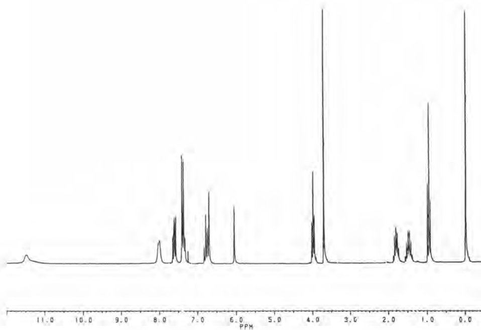
Fig 14 The 1 H-NMR spectrum of Compound 30
