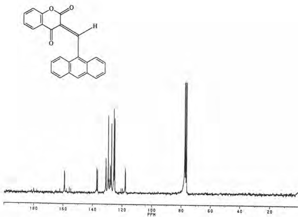
Fig 43 The ^{13}\text{C} -NMR spectrum of Compound 54
