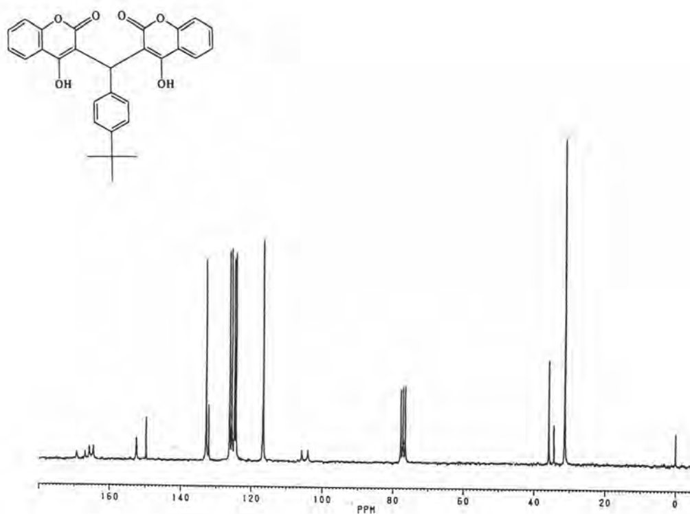
Fig 3 The ^{13}\text{C} -NMR spectrum of Compound 17
