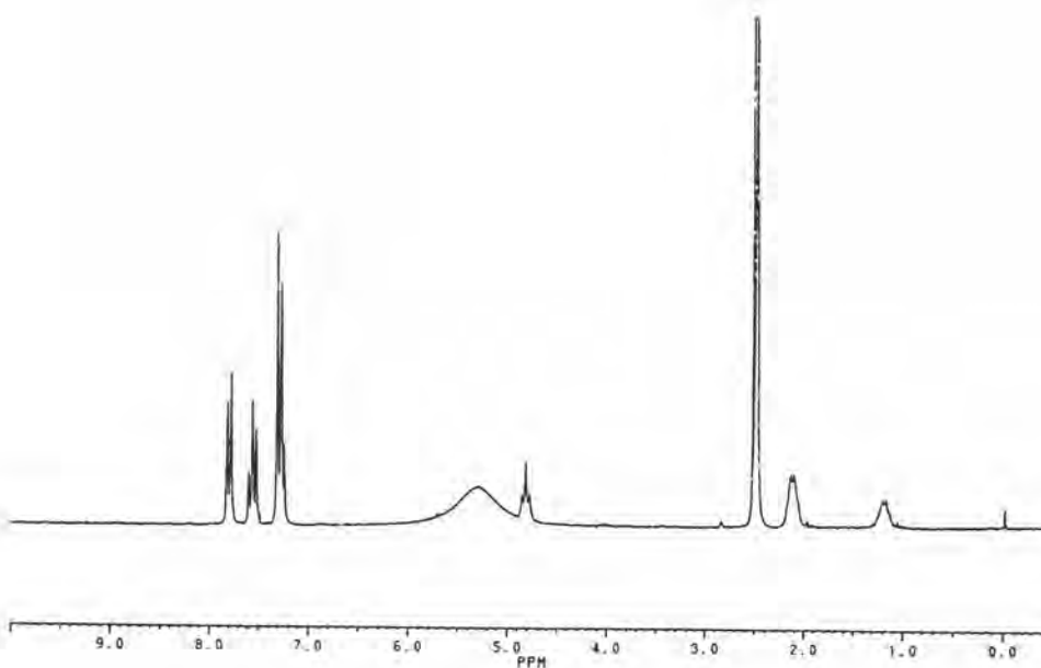
Fig 38 The 1 H-NMR spectrum of Compound 50
