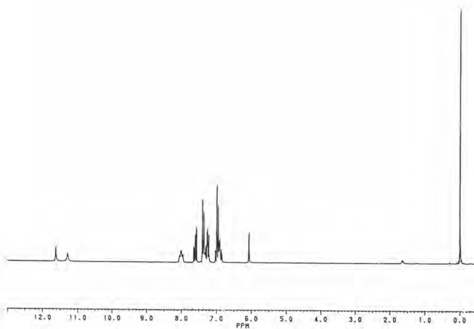
Fig 6 The 1 H-NMR spectrum of Compound 23
