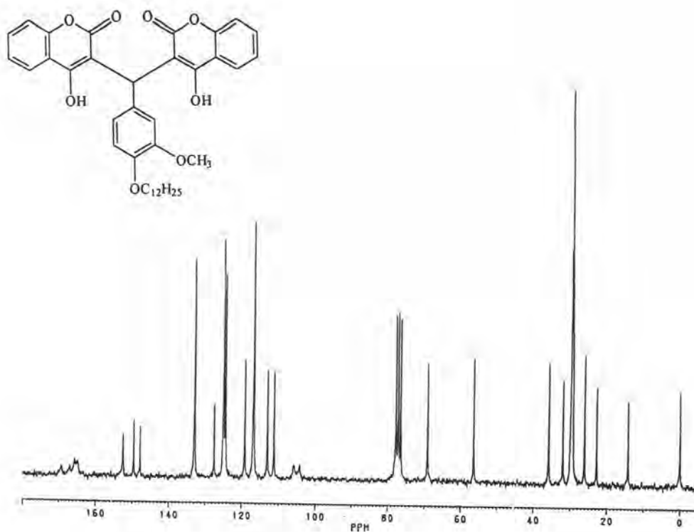
Fig 27 The ^{13}\text{C} -NMR spectrum of Compound 33
