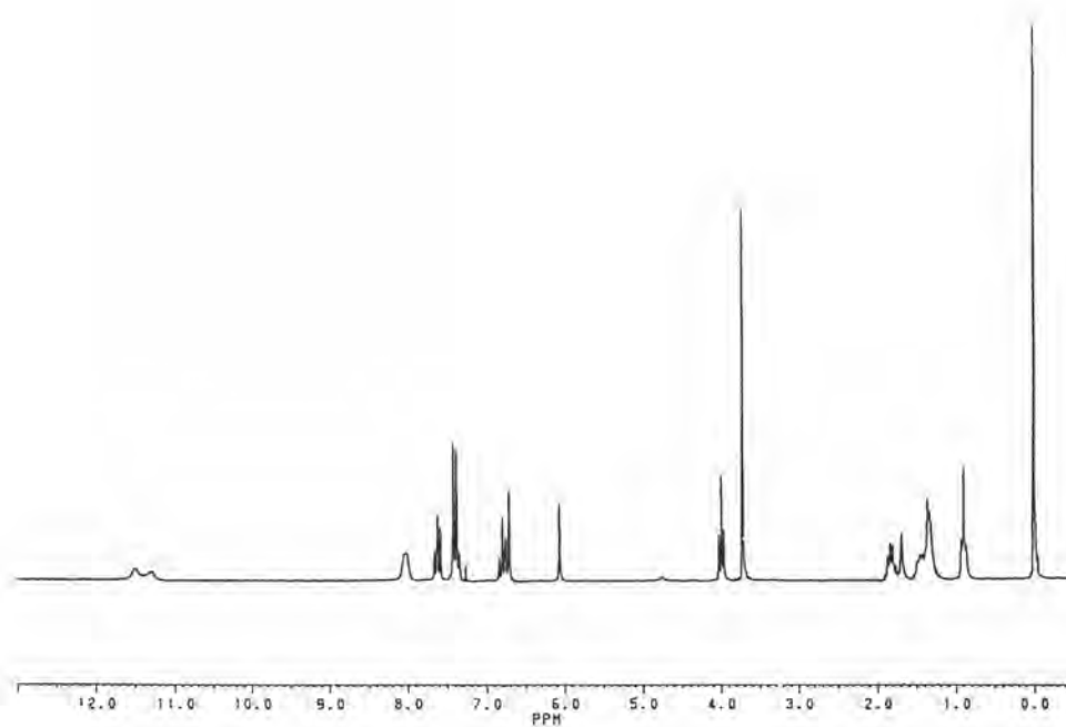
Fig 18 The 1 H-NMR spectrum of Compound 31
