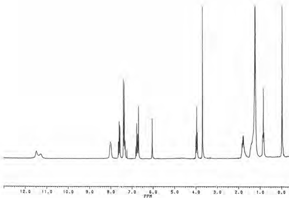
Fig 26 The 1 H-NMR spectrum of Compound 33
