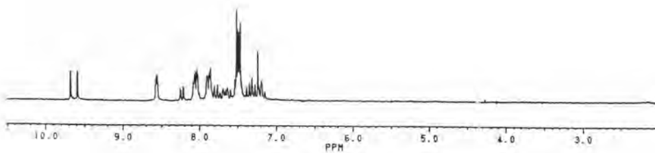
Fig 42 The 1 H-NMR spectrum of Compound 54
