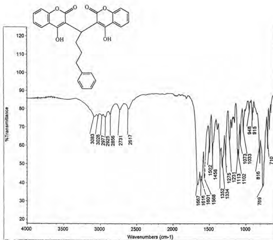
Fig 33 The FT-IR spectrum of Compound 44
