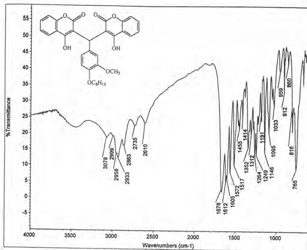
Fig 17 The FT-IR spectrum of Compound 31
