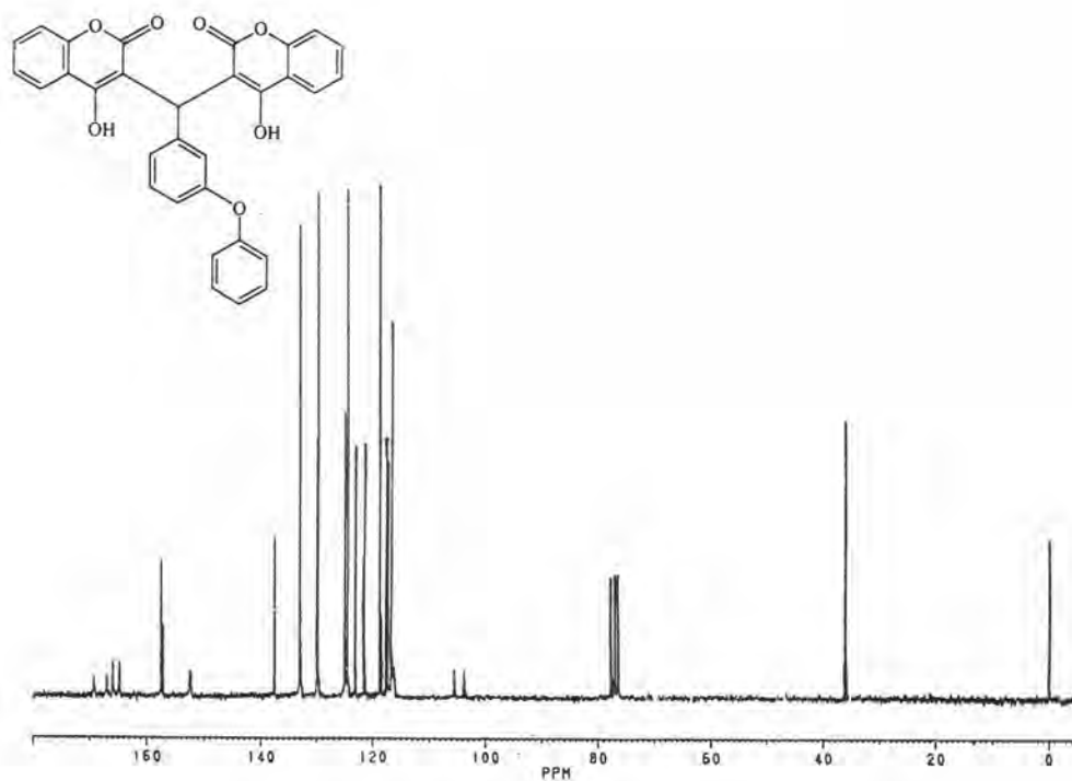
Fig 7 The ^{13}\text{C} -NMR spectrum of Compound 23
