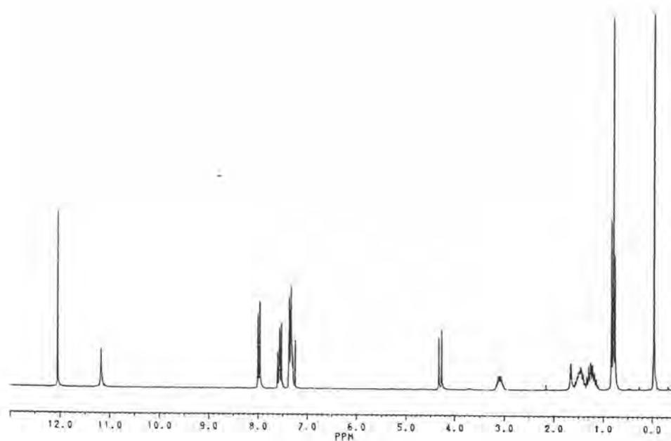
Fig 30 The 1 H-NMR spectrum of Compound 38
