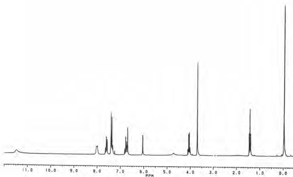
Fig 10 The 1 H-NMR spectrum of Compound 29
