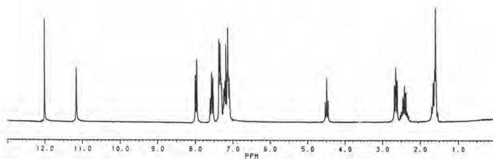
Fig 34 The 1 H-NMR spectrum of Compound 44
