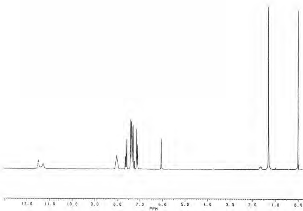
Fig 2 The 1 H-NMR spectrum of Compound 17
