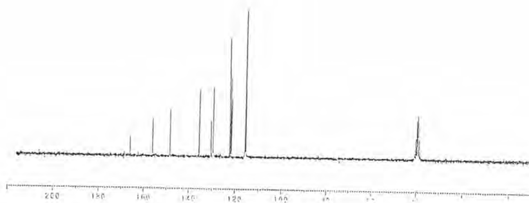
Figure A3 The ^{13}\text{C} -NMR spectrum of compound T1
