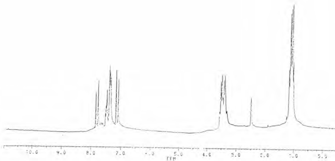
Figure A32 The 1 H-NMR spectrum of compound T11
