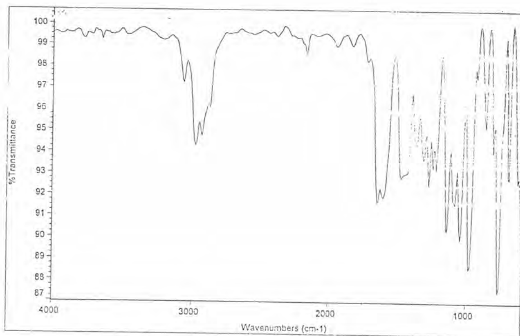
Figure A31 The IR spectrum of compound T11
