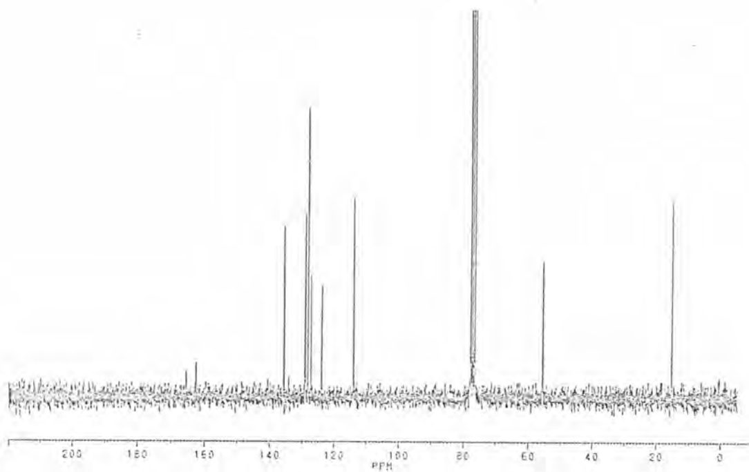
Figure A15 The ^{13}\text{C} -NMR spectrum of compound T5
