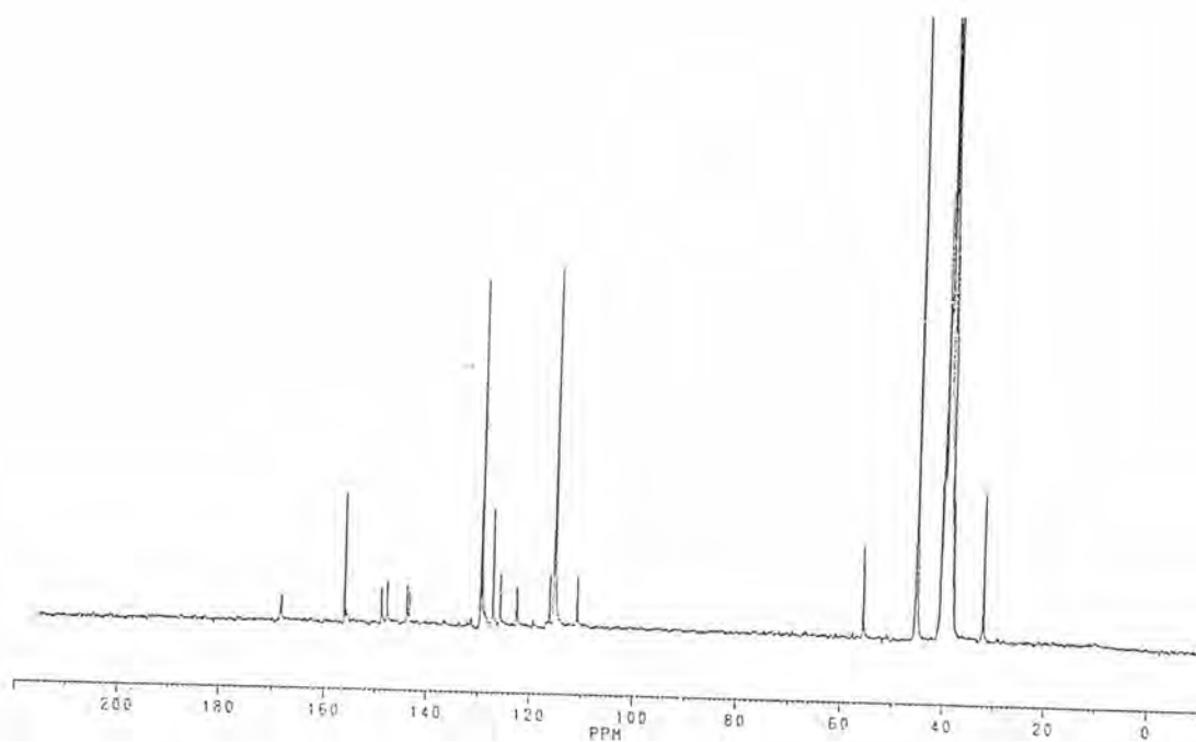
Figure A24 The ^{13}\text{C} -NMR spectrum of compound T8
