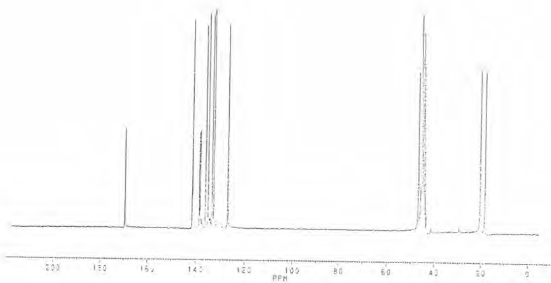
Figure A33 The ^{13}\text{C} -NMR spectrum of compound T11
