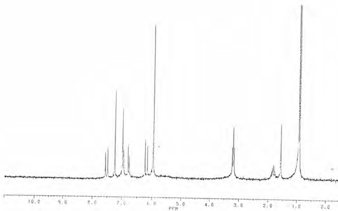
Figure A29 The 1 H-NMR spectrum of compound T10
