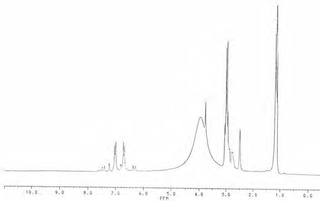
Figure A23 The 1 H-NMR spectrum of compound T8
