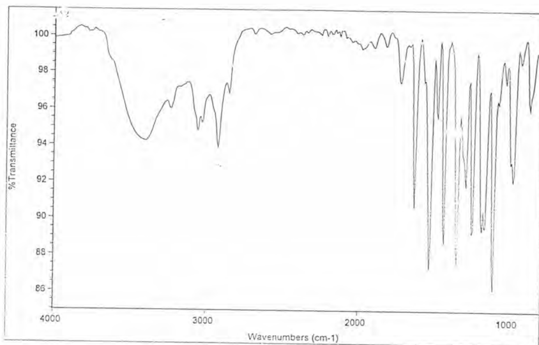
Figure A25 The IR spectrum of compound T9
