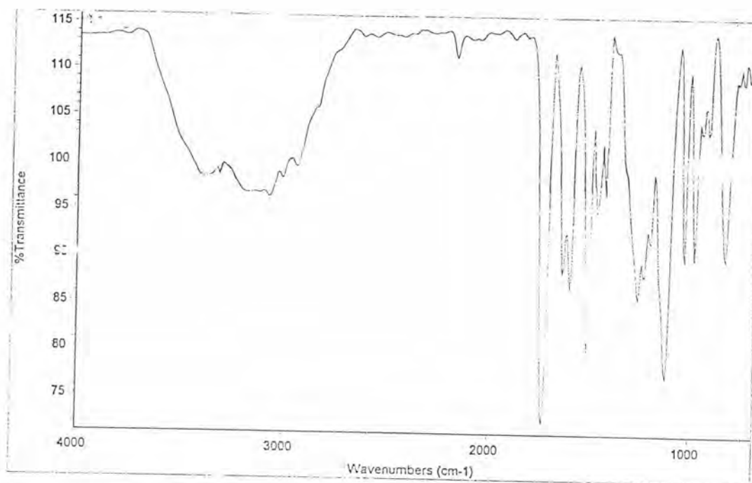
Figure A22 The IR spectrum of compound T8
