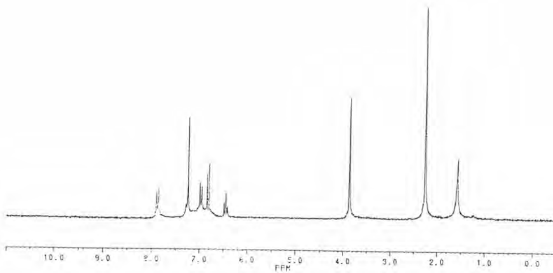
Figure A14 The 1 H-NMR spectrum of compound T5
