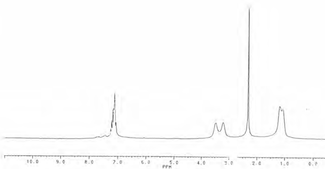
Figure A5 The 1 H-NMR spectrum of compound T2
