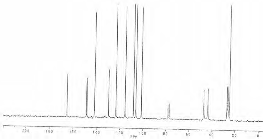
Figure A18 The ^{13}\text{C} -NMR spectrum of compound T6
