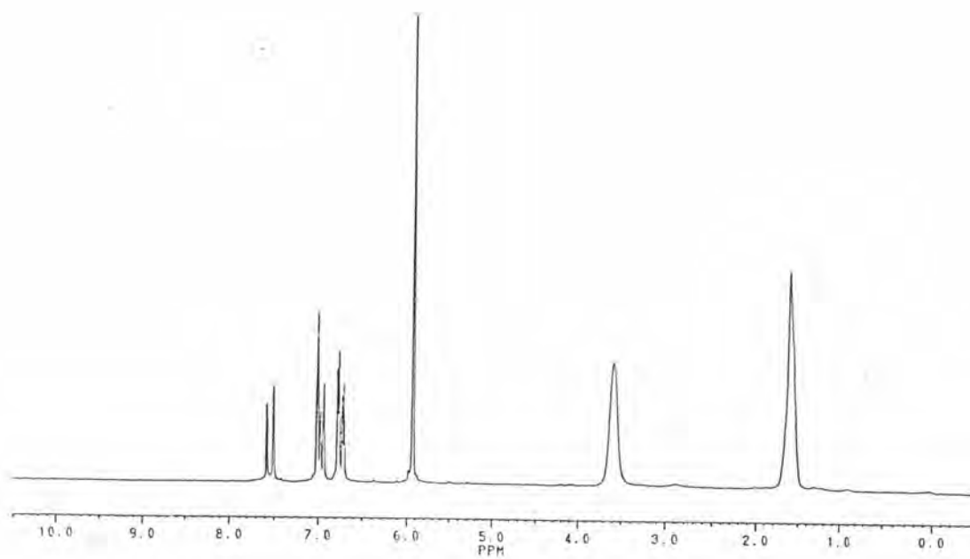
Figure A17 The 1 H-NMR spectrum of compound T6
