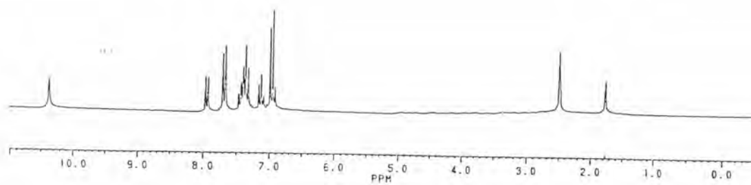
Figure A2 The 1 H-NMR spectrum of compound T1
