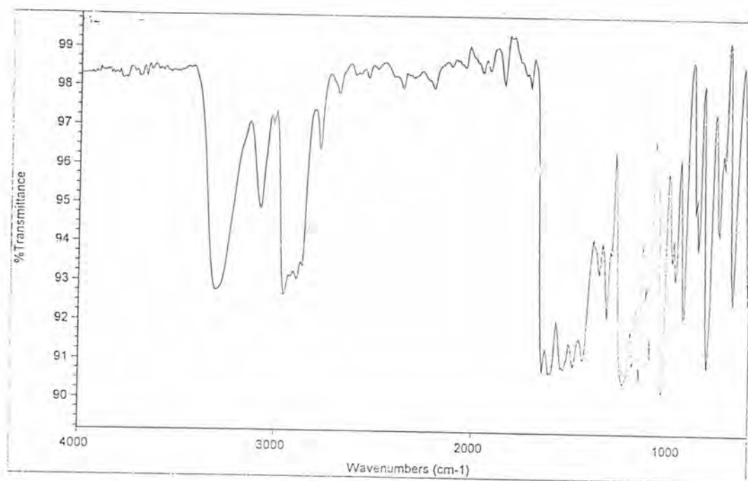
Figure A28 The IR spectrum of compound T10
