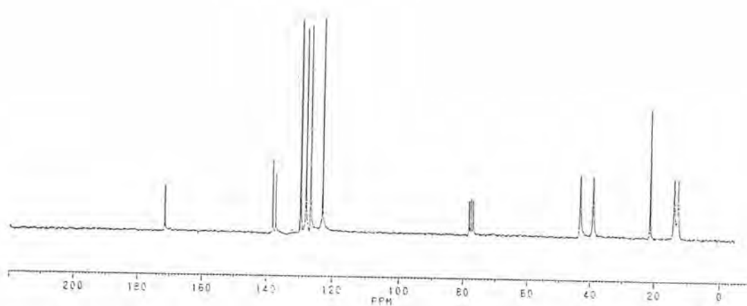
Figure A6 The ^{13}\text{C} -NMR spectrum of compound T2
