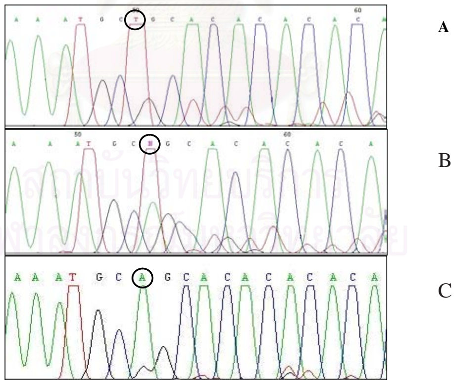
Figure 2. Chromatogram of DNA sequences in homozygous of +874T, heterozygous +874T/A and homozygous of +874A. Homozygous of +874T from sample N7 (A), heterozygous +874T/A from sample N9 (B) and homozygous of +874A from sample N5 (C).
