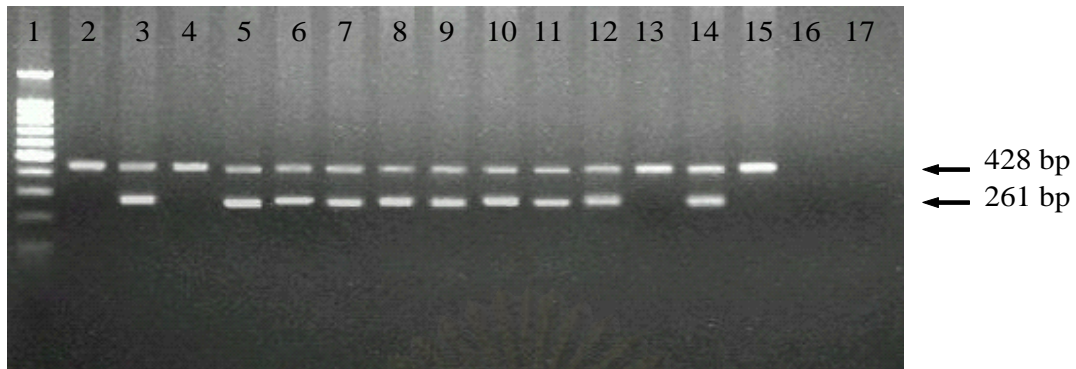
Figure 1. The representative result from samples with homozygous of +874T, heterozygous +874T/A and homozygous of +874A. Lane 1 is 100 bp molecular marker. Lane 2-5 (2-3 sample N7 and 4-5 sample N14) are homozygous of +874T. Lane 6-11 (6-7 sample N9, 8-9 sample N11 and 10-11 sample N17) are heterozygous +874T/A. Lane 12-15 (12-13 sample N5 and 4-15 sample N6) are homozygous of +874A. Lane 16-17 are Negative control of in each specific primer (NA is Negative control of +874A allele specific primer and NT is Negative control of +874T allele specific primer).
