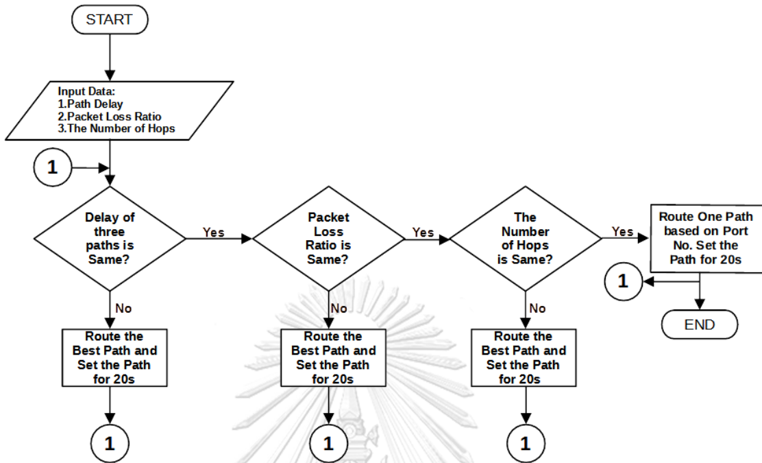
Figure 4.2: Flowchart diagram for routing algorithm
